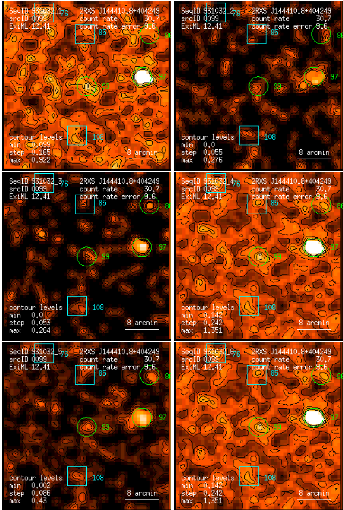
Figure 99: RASS 931032: detection 0099: band rate images, Gaussian filter: (1) PSPC channels 11 – 41, (2) 52 – 90, (3) 91 – 201, (4) 11 – 235, (5) 52 – 201, (6) 11 – 201. Broad band rates in counts/ks. Band rate contour levels in counts/ks/arcmin 2 .
