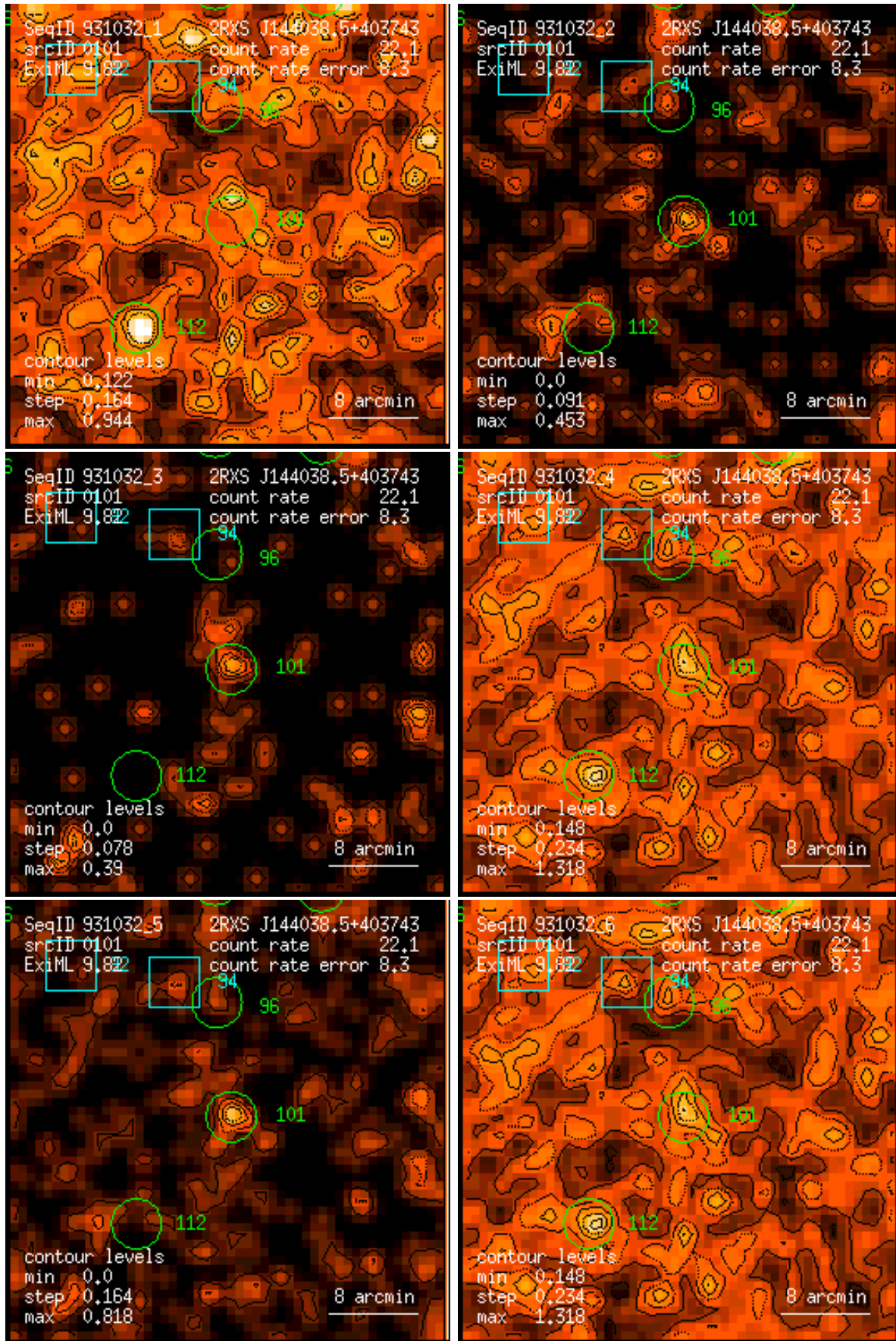
Figure 101: RASS 931032: detection 0101: band rate images, Gaussian filter: (1) PSPC channels 11 – 41, (2) 52 – 90, (3) 91 – 201, (4) 11 – 235, (5) 52 – 201, (6) 11 – 201. Broad band rates in counts/ks. Band rate contour levels in counts/ks/arcmin 2 .
