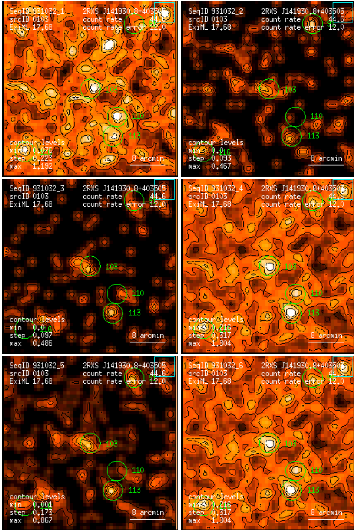
Figure 103: RASS 931032: detection 0103: band rate images, Gaussian filter: (1) PSPC channels 11 – 41, (2) 52 – 90, (3) 91 – 201, (4) 11 – 235, (5) 52 – 201, (6) 11 – 201. Broad band rates in counts/ks. Band rate contour levels in counts/ks/arcmin 2 .
