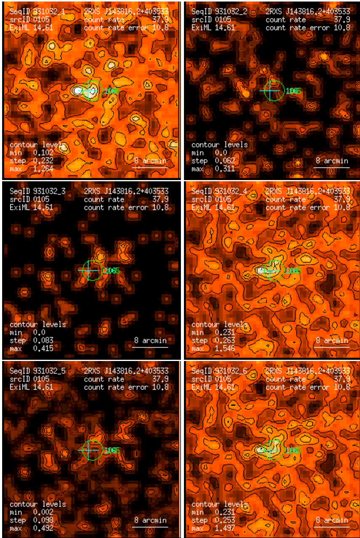
Figure 105: RASS 931032: detection 0105: band rate images, Gaussian filter: (1) PSPC channels 11 – 41, (2) 52 – 90, (3) 91 – 201, (4) 11 – 235, (5) 52 – 201, (6) 11 – 201. Broad band rates in counts/ks. Band rate contour levels in counts/ks/arcmin 2 .
