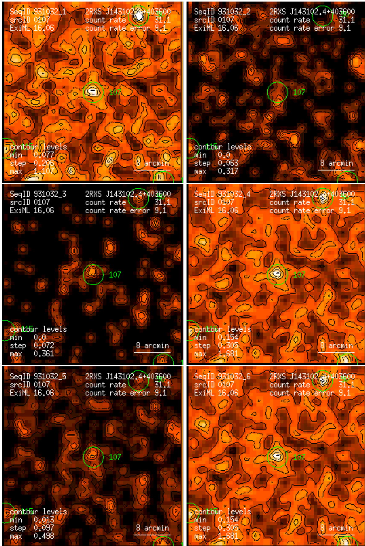
Figure 107: RASS 931032: detection 0107: band rate images, Gaussian filter: (1) PSPC channels 11 – 41, (2) 52 – 90, (3) 91 – 201, (4) 11 – 235, (5) 52 – 201, (6) 11 – 201. Broad band rates in counts/ks. Band rate contour levels in counts/ks/arcmin 2 .
