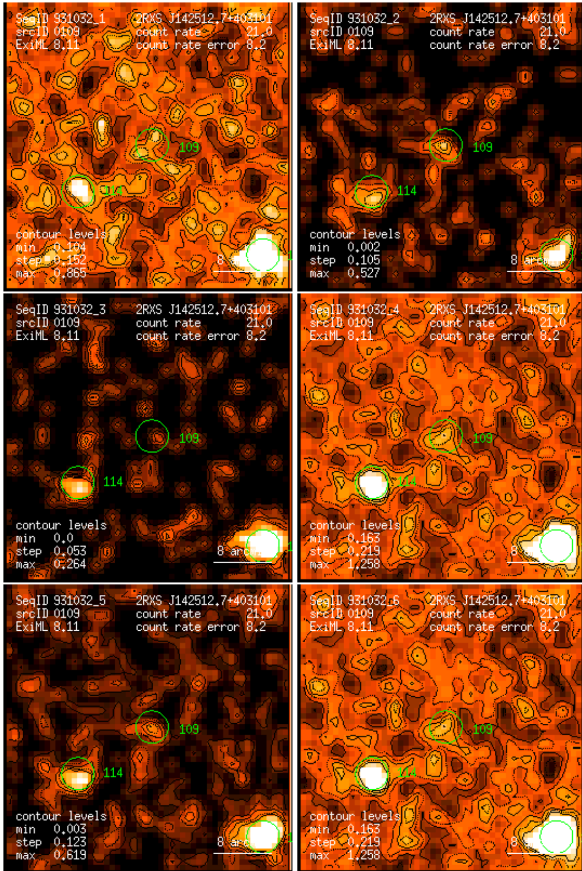
Figure 109: RASS 931032: detection 0109: band rate images, Gaussian filter: (1) PSPC channels 11 – 41, (2) 52 – 90, (3) 91 – 201, (4) 11 – 235, (5) 52 – 201, (6) 11 – 201. Broad band rates in counts/ks. Band rate contour levels in counts/ks/arcmin 2 .
