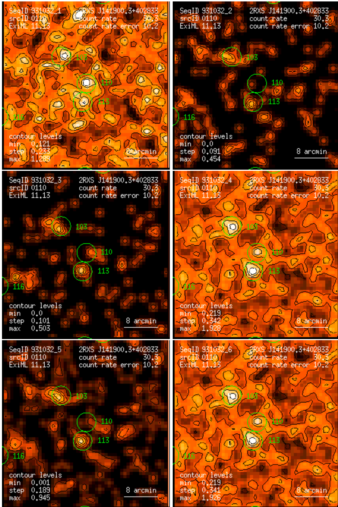
Figure 110: RASS 931032: detection 0110: band rate images, Gaussian filter: (1) PSPC channels 11 – 41, (2) 52 – 90, (3) 91 – 201, (4) 11 – 235, (5) 52 – 201, (6) 11 – 201. Broad band rates in counts/ks. Band rate contour levels in counts/ks/arcmin 2 .
