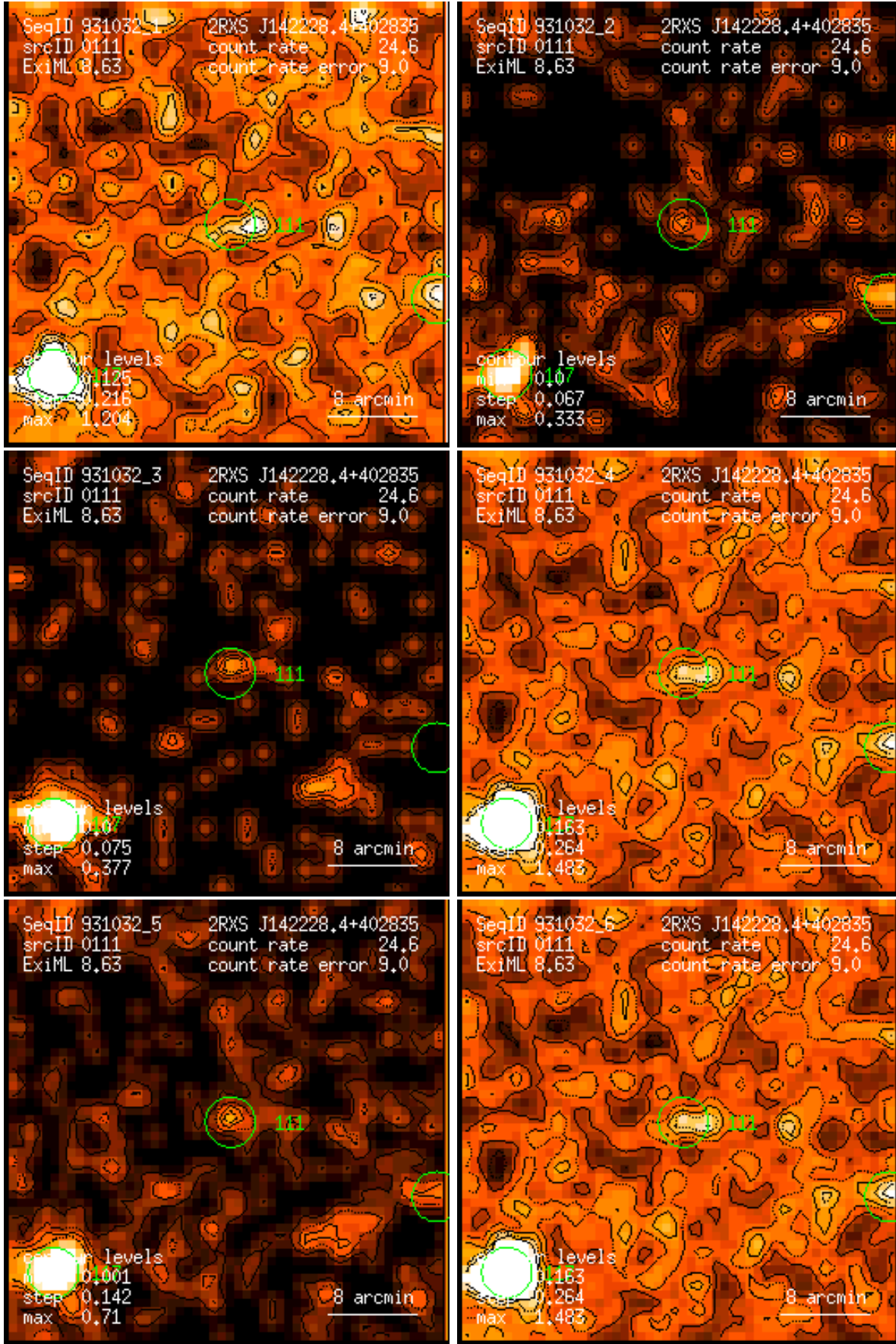
Figure 111: RASS 931032: detection 0111: band rate images, Gaussian filter: (1) PSPC channels 11 – 41, (2) 52 – 90, (3) 91 – 201, (4) 11 – 235, (5) 52 – 201, (6) 11 – 201. Broad band rates in counts/ks. Band rate contour levels in counts/ks/arcmin 2 .
