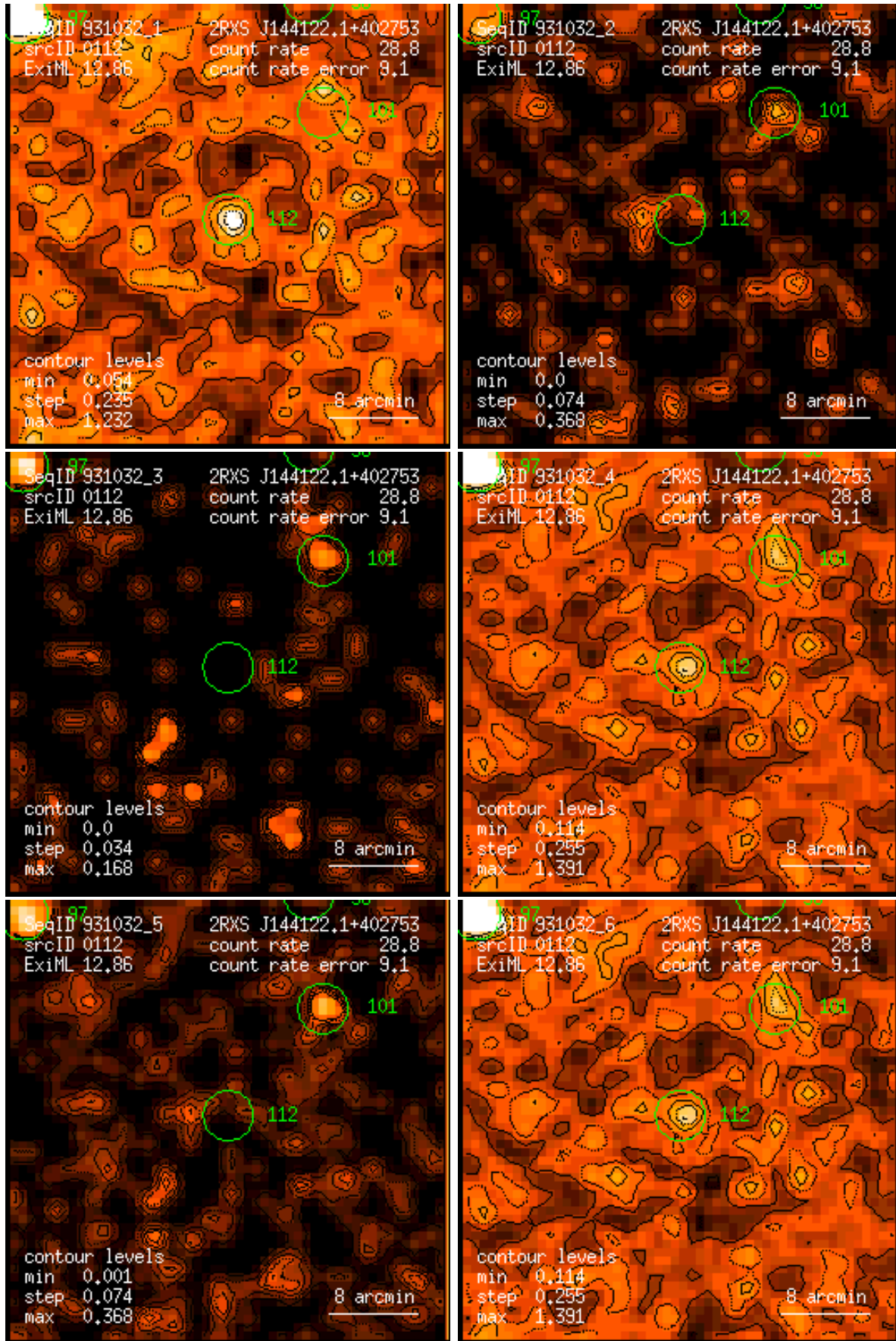
Figure 112: RASS 931032: detection 0112: band rate images, Gaussian filter: (1) PSPC channels 11 – 41, (2) 52 – 90, (3) 91 – 201, (4) 11 – 235, (5) 52 – 201, (6) 11 – 201. Broad band rates in counts/ks. Band rate contour levels in counts/ks/arcmin 2 .
