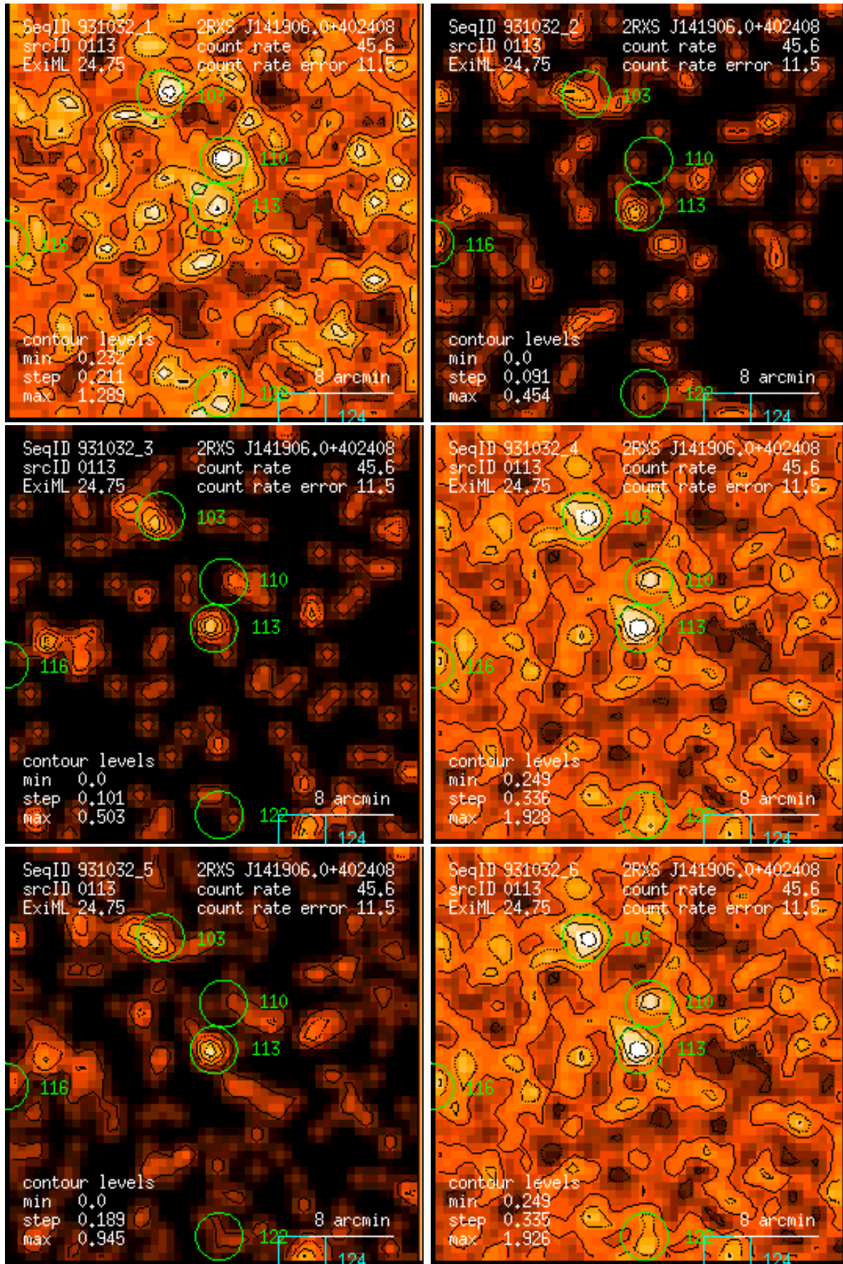
Figure 113: RASS 931032: detection 0113: band rate images, Gaussian filter: (1) PSPC channels 11 – 41, (2) 52 – 90, (3) 91 – 201, (4) 11 – 235, (5) 52 – 201, (6) 11 – 201. Broad band rates in counts/ks. Band rate contour levels in counts/ks/arcmin 2 .
