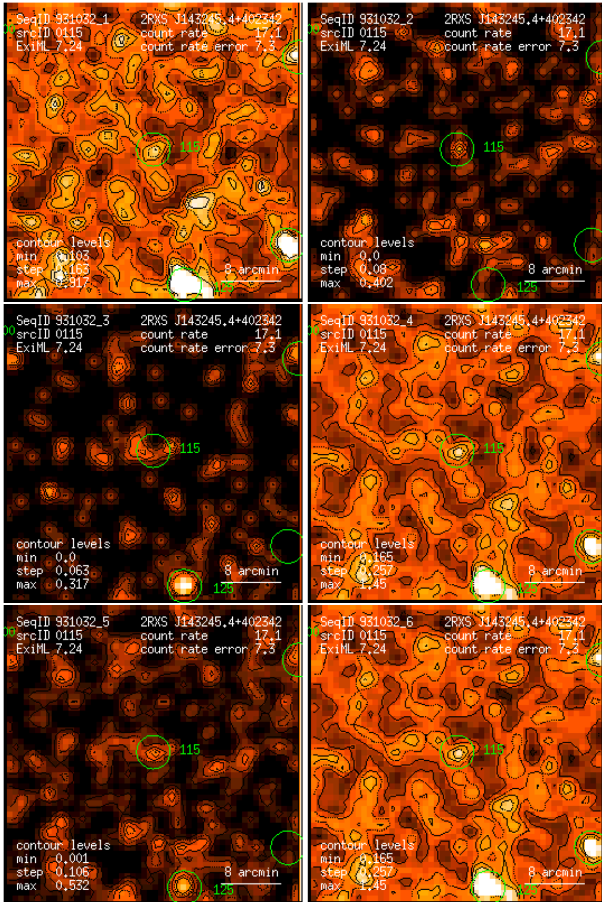
Figure 115: RASS 931032: detection 0115: band rate images, Gaussian filter: (1) PSPC channels 11 – 41, (2) 52 – 90, (3) 91 – 201, (4) 11 – 235, (5) 52 – 201, (6) 11 – 201. Broad band rates in counts/ks. Band rate contour levels in counts/ks/arcmin 2 .
