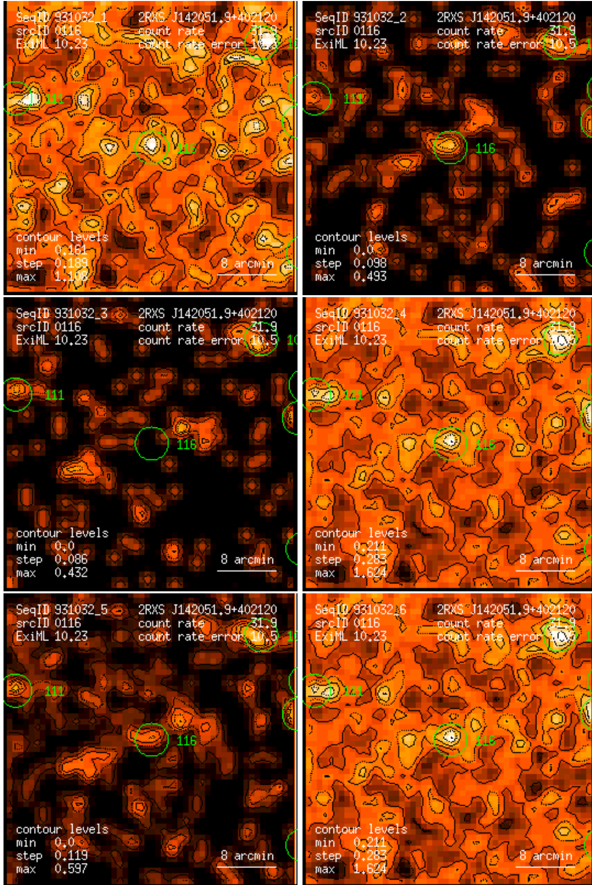
Figure 116: RASS 931032: detection 0116: band rate images, Gaussian filter: (1) PSPC channels 11 – 41, (2) 52 – 90, (3) 91 – 201, (4) 11 – 235, (5) 52 – 201, (6) 11 – 201. Broad band rates in counts/ks. Band rate contour levels in counts/ks/arcmin 2 .
