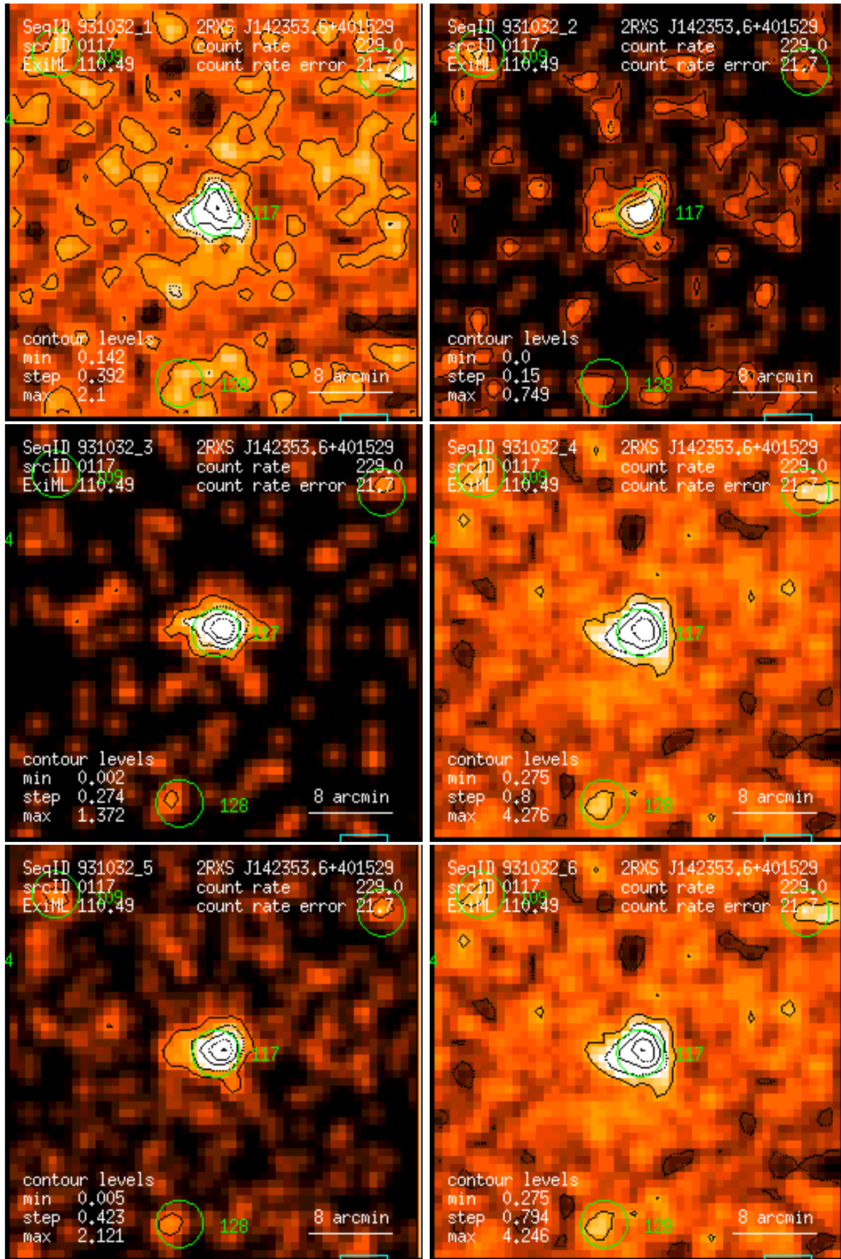
Figure 117: RASS 931032: detection 0117: band rate images, Gaussian filter: (1) PSPC channels 11 – 41, (2) 52 – 90, (3) 91 – 201, (4) 11 – 235, (5) 52 – 201, (6) 11 – 201. Broad band rates in counts/ks. Band rate contour levels in counts/ks/arcmin 2 .
