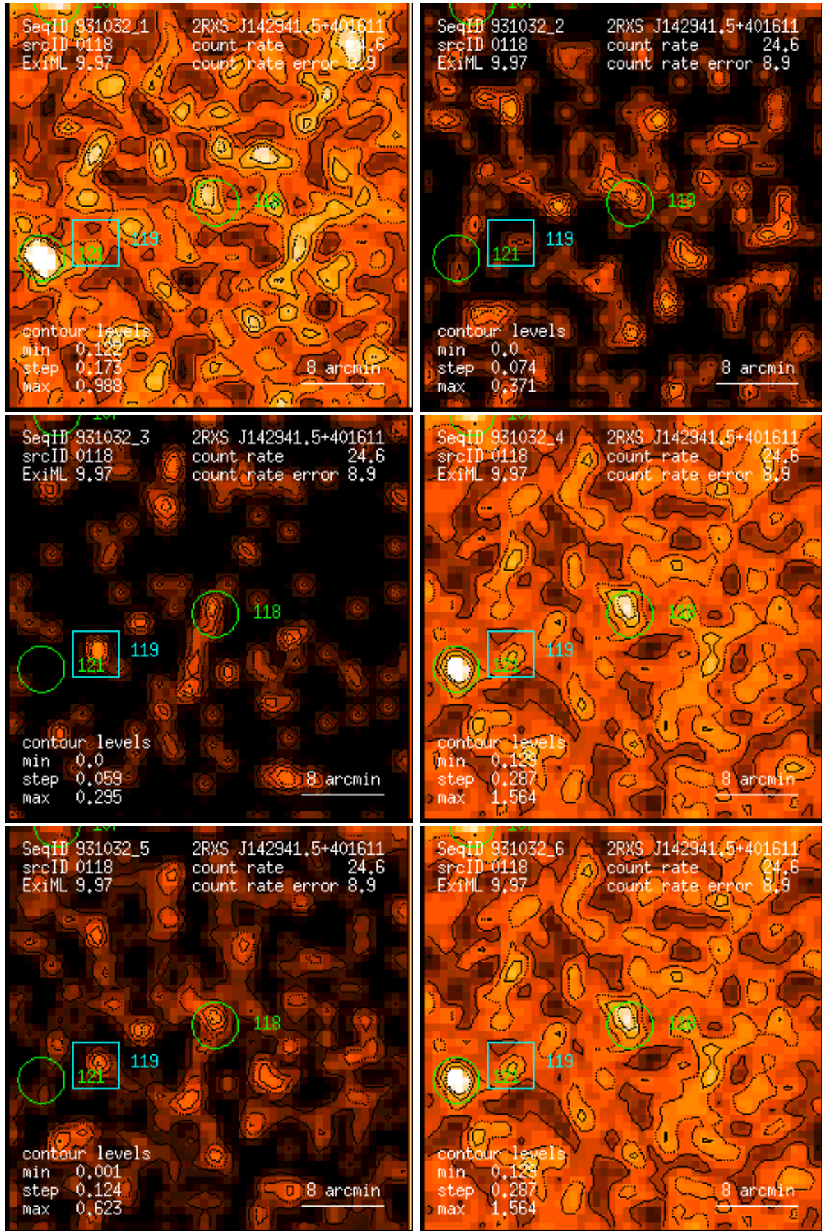
Figure 118: RASS 931032: detection 0118: band rate images, Gaussian filter: (1) PSPC channels 11 – 41, (2) 52 – 90, (3) 91 – 201, (4) 11 – 235, (5) 52 – 201, (6) 11 – 201. Broad band rates in counts/ks. Band rate contour levels in counts/ks/arcmin 2 .
