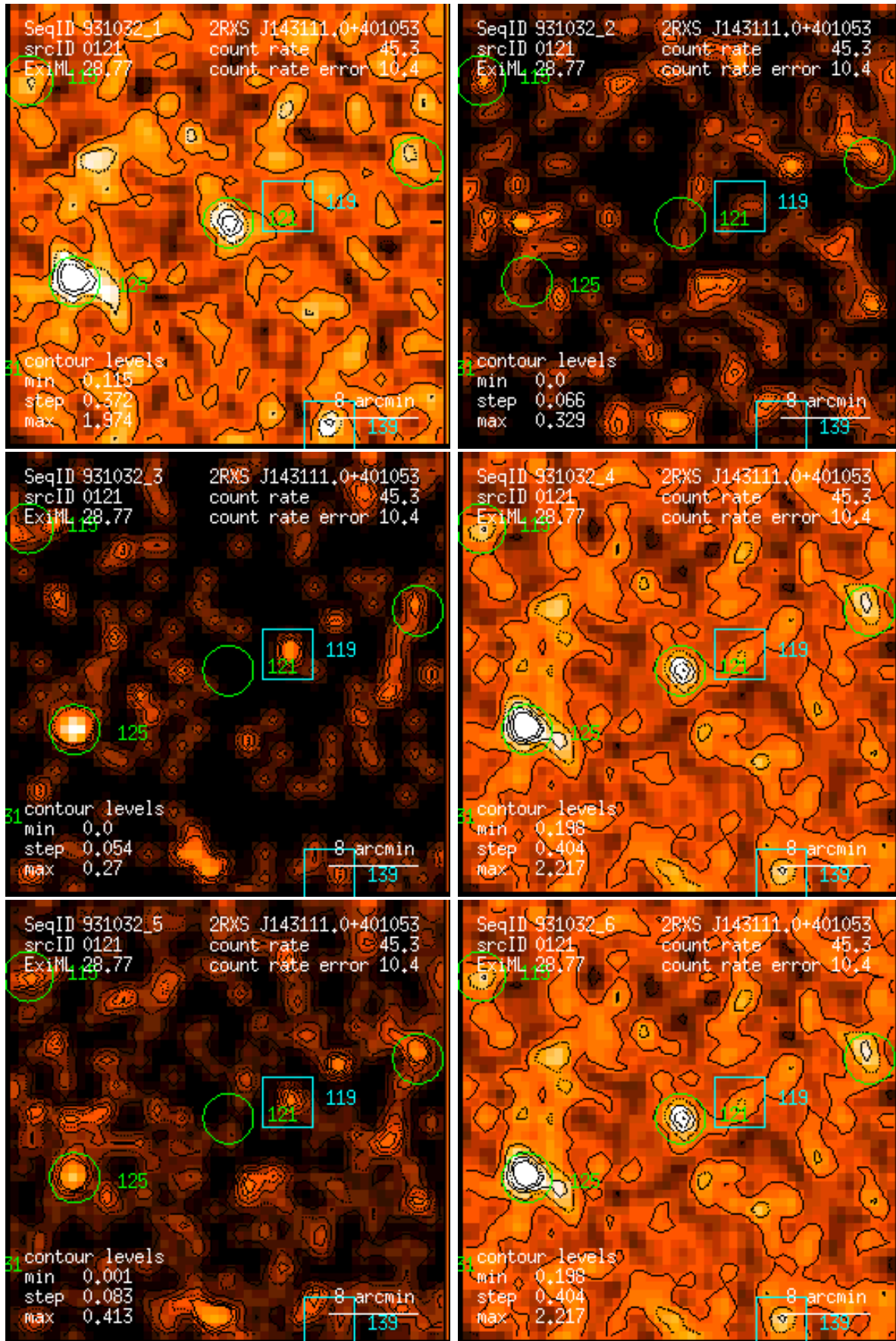
Figure 121: RASS 931032: detection 0121: band rate images, Gaussian filter: (1) PSPC channels 11 – 41, (2) 52 – 90, (3) 91 – 201, (4) 11 – 235, (5) 52 – 201, (6) 11 – 201. Broad band rates in counts/ks. Band rate contour levels in counts/ks/arcmin 2 .
