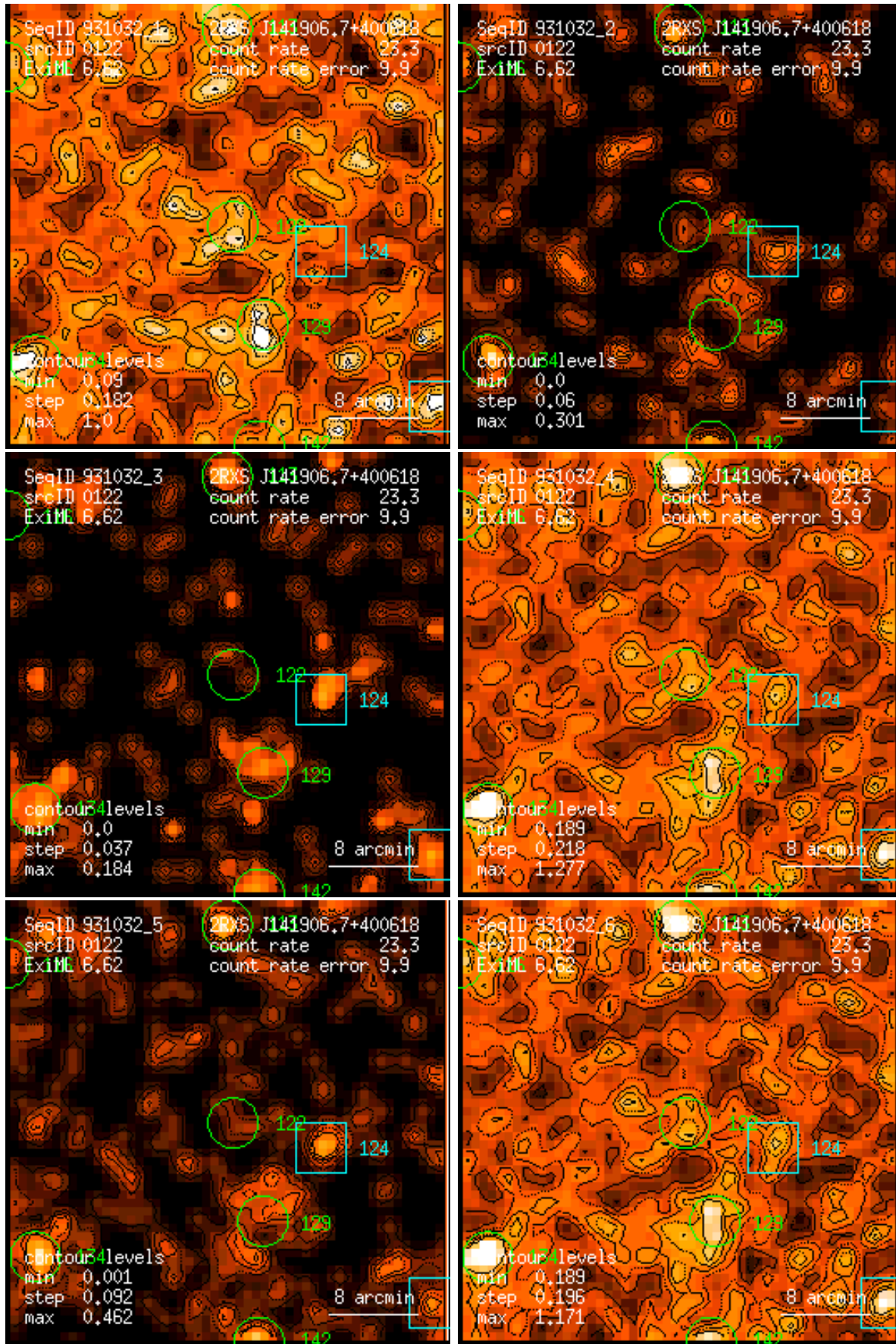
Figure 122: RASS 931032: detection 0122: band rate images, Gaussian filter: (1) PSPC channels 11 – 41, (2) 52 – 90, (3) 91 – 201, (4) 11 – 235, (5) 52 – 201, (6) 11 – 201. Broad band rates in counts/ks. Band rate contour levels in counts/ks/arcmin 2 .
