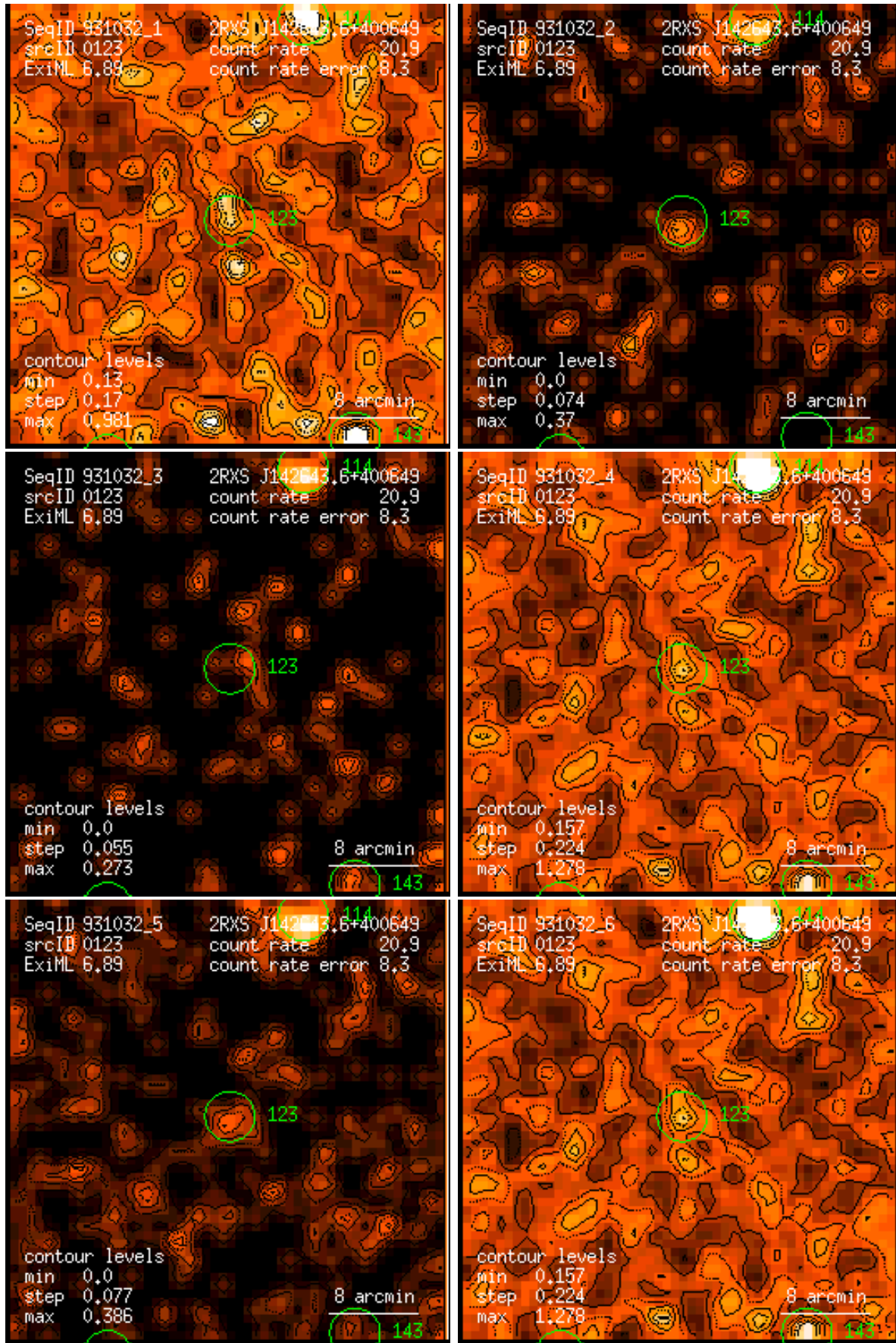
Figure 123: RASS 931032: detection 0123: band rate images, Gaussian filter: (1) PSPC channels 11 – 41, (2) 52 – 90, (3) 91 – 201, (4) 11 – 235, (5) 52 – 201, (6) 11 – 201. Broad band rates in counts/ks. Band rate contour levels in counts/ks/arcmin 2 .
