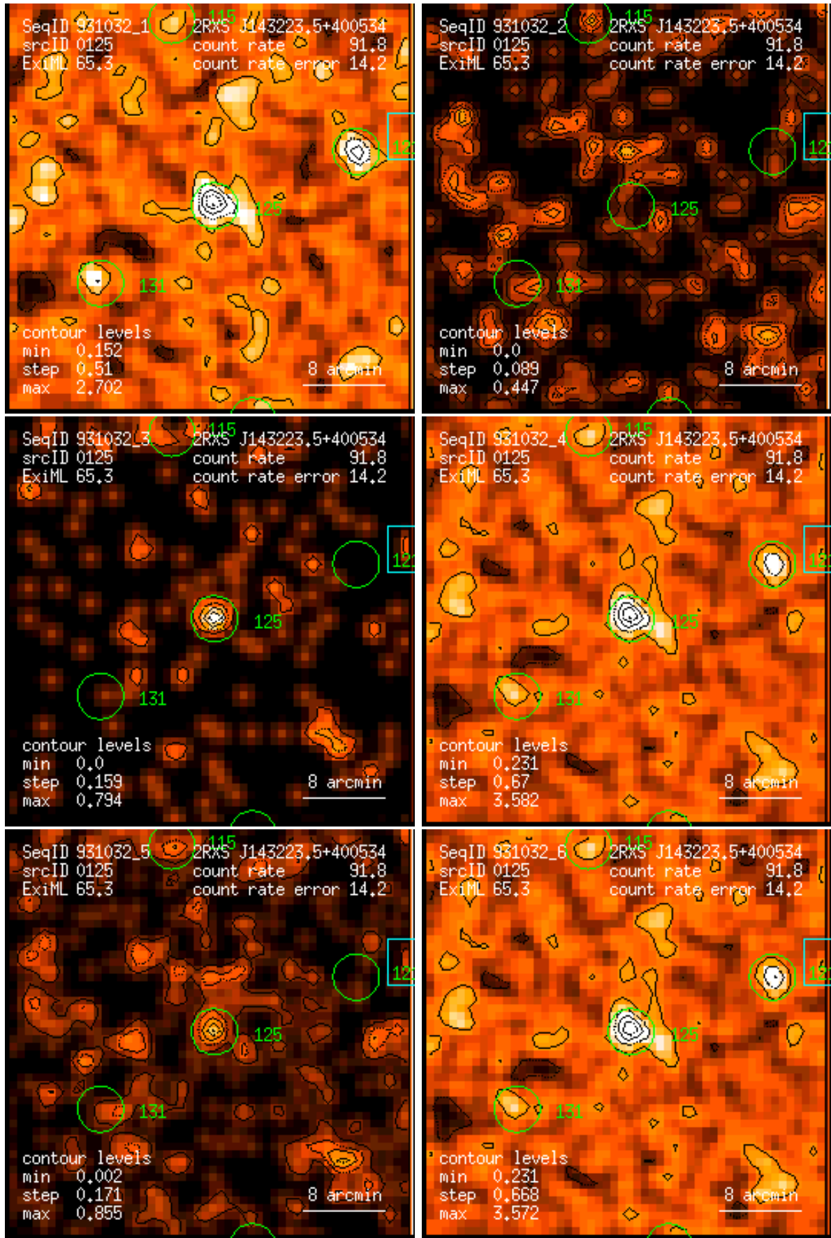
Figure 125: RASS 931032: detection 0125: band rate images, Gaussian filter: (1) PSPC channels 11 – 41, (2) 52 – 90, (3) 91 – 201, (4) 11 – 235, (5) 52 – 201, (6) 11 – 201. Broad band rates in counts/ks. Band rate contour levels in counts/ks/arcmin 2 .
