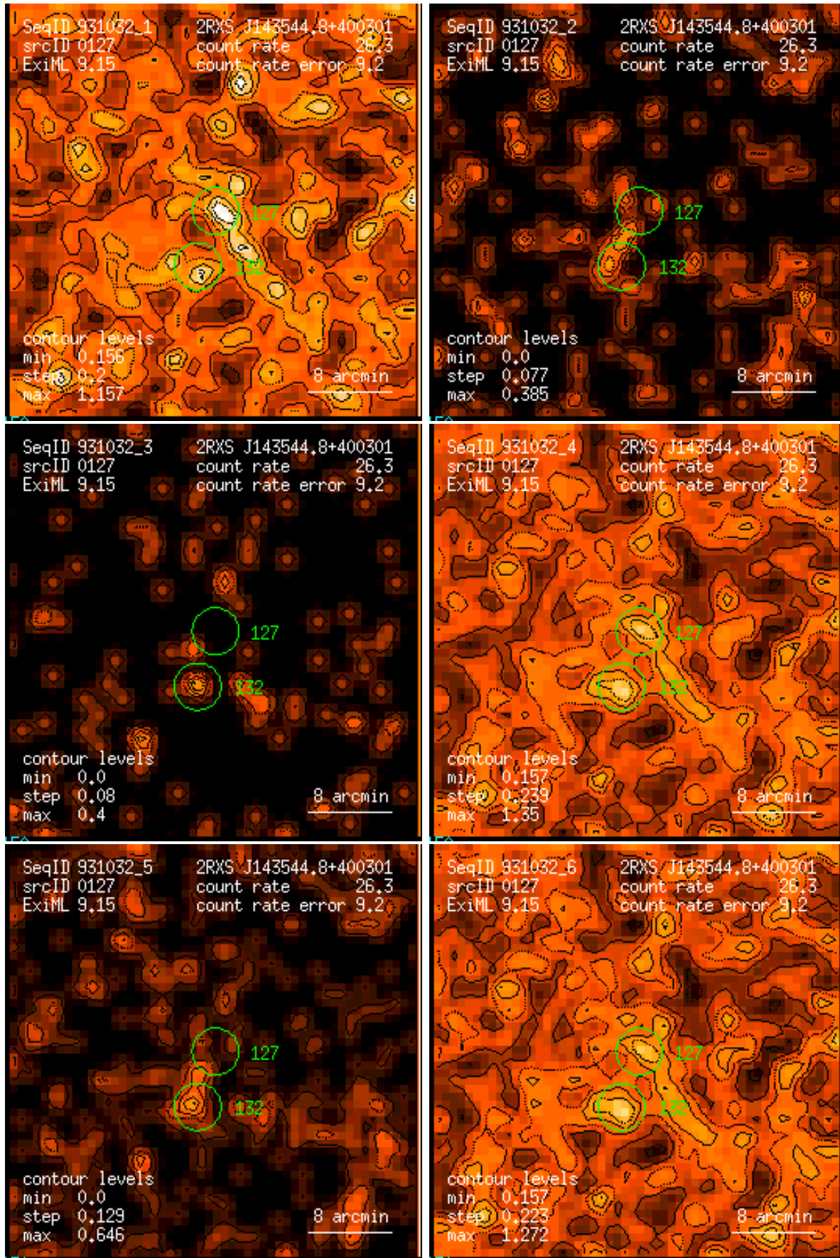
Figure 127: RASS 931032: detection 0127: band rate images, Gaussian filter: (1) PSPC channels 11 – 41, (2) 52 – 90, (3) 91 – 201, (4) 11 – 235, (5) 52 – 201, (6) 11 – 201. Broad band rates in counts/ks. Band rate contour levels in counts/ks/arcmin 2 .
