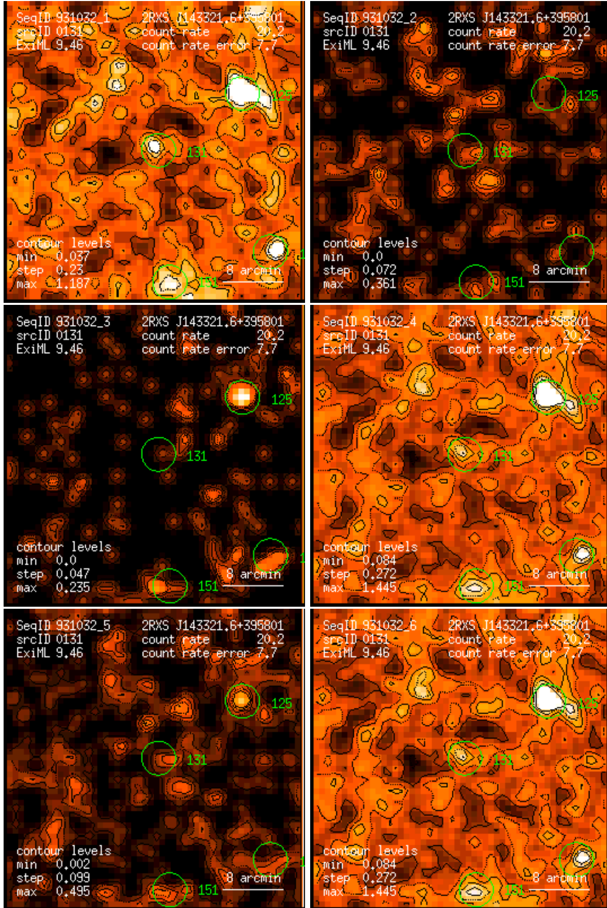
Figure 131: RASS 931032: detection 0131: band rate images, Gaussian filter: (1) PSPC channels 11 – 41, (2) 52 – 90, (3) 91 – 201, (4) 11 – 235, (5) 52 – 201, (6) 11 – 201. Broad band rates in counts/ks. Band rate contour levels in counts/ks/arcmin 2 .
