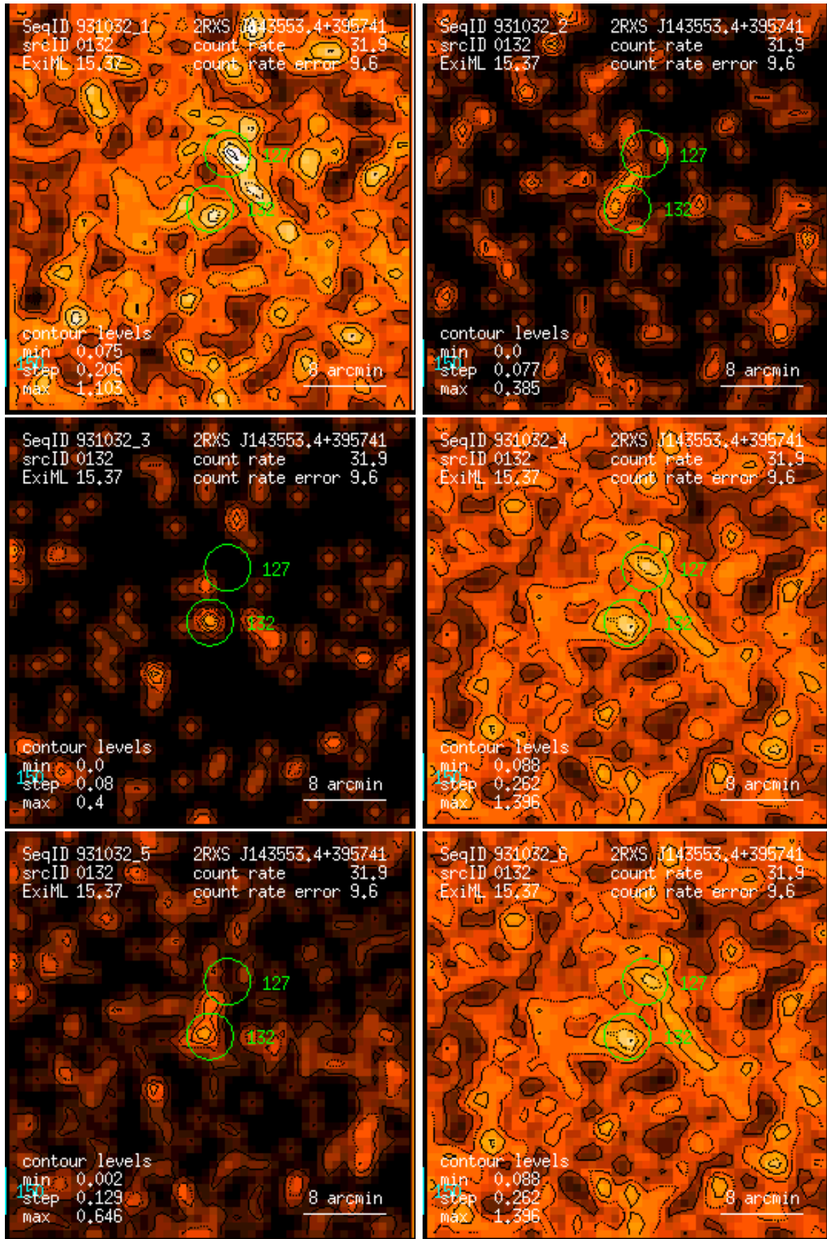
Figure 132: RASS 931032: detection 0132: band rate images, Gaussian filter: (1) PSPC channels 11 – 41, (2) 52 – 90, (3) 91 – 201, (4) 11 – 235, (5) 52 – 201, (6) 11 – 201. Broad band rates in counts/ks. Band rate contour levels in counts/ks/arcmin 2 .
