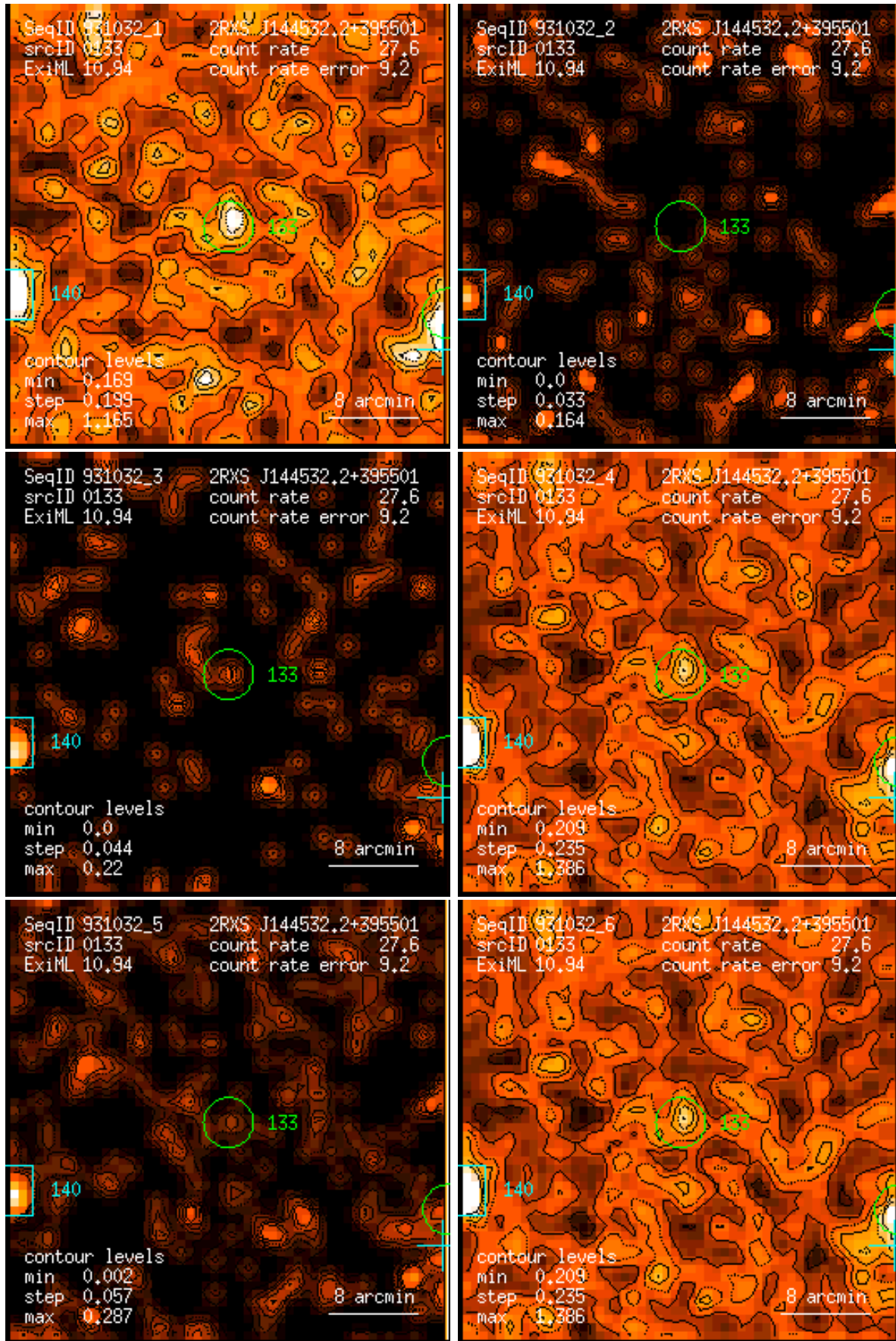
Figure 133: RASS 931032: detection 0133: band rate images, Gaussian filter: (1) PSPC channels 11 – 41, (2) 52 – 90, (3) 91 – 201, (4) 11 – 235, (5) 52 – 201, (6) 11 – 201. Broad band rates in counts/ks. Band rate contour levels in counts/ks/arcmin 2 .
