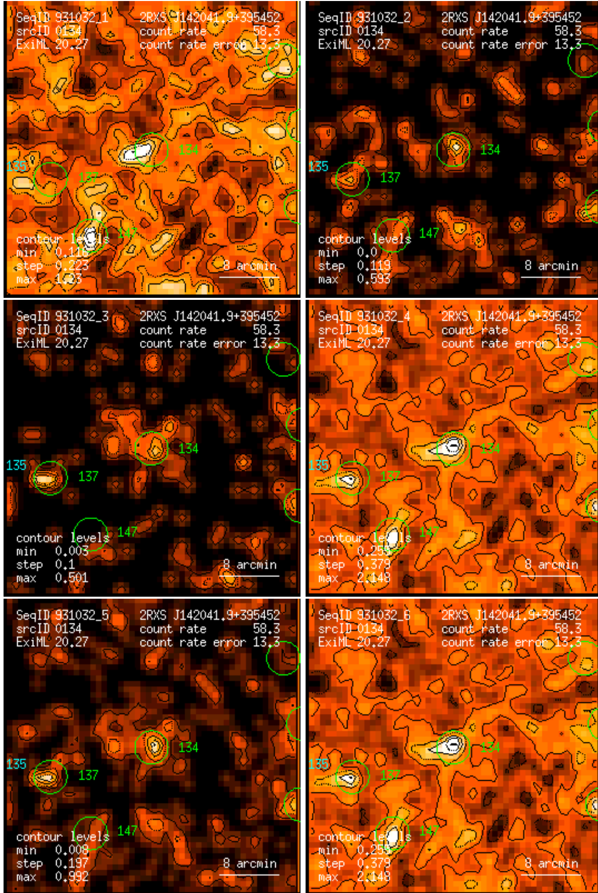
Figure 134: RASS 931032: detection 0134: band rate images, Gaussian filter: (1) PSPC channels 11 – 41, (2) 52 – 90, (3) 91 – 201, (4) 11 – 235, (5) 52 – 201, (6) 11 – 201. Broad band rates in counts/ks. Band rate contour levels in counts/ks/arcmin 2 .
