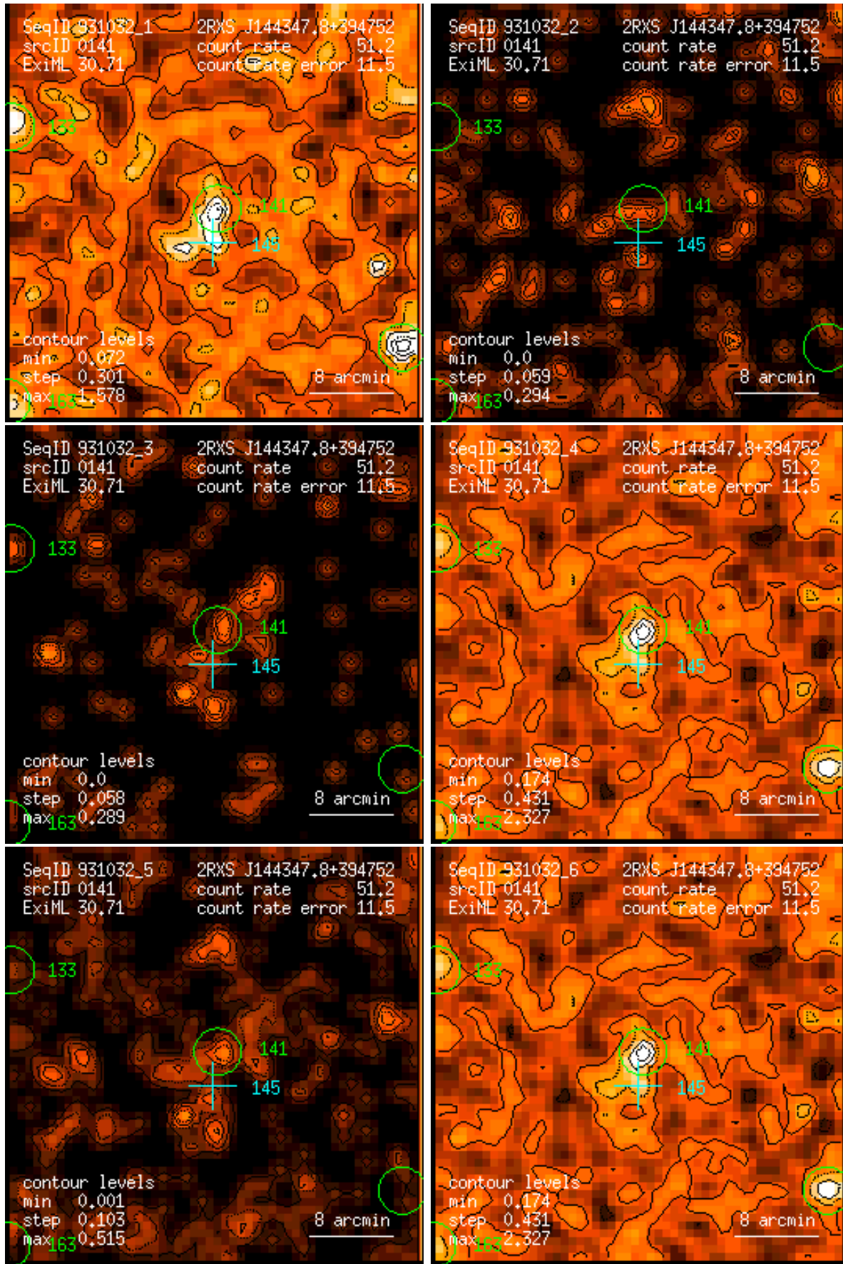
Figure 141: RASS 931032: detection 0141: band rate images, Gaussian filter: (1) PSPC channels 11 – 41, (2) 52 – 90, (3) 91 – 201, (4) 11 – 235, (5) 52 – 201, (6) 11 – 201. Broad band rates in counts/ks. Band rate contour levels in counts/ks/arcmin 2 .
