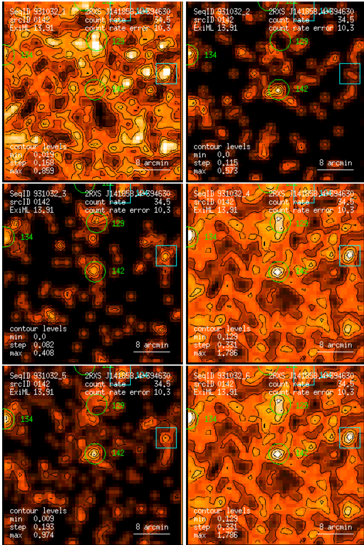
Figure 142: RASS 931032: detection 0142: band rate images, Gaussian filter: (1) PSPC channels 11 – 41, (2) 52 – 90, (3) 91 – 201, (4) 11 – 235, (5) 52 – 201, (6) 11 – 201. Broad band rates in counts/ks. Band rate contour levels in counts/ks/arcmin 2 .
