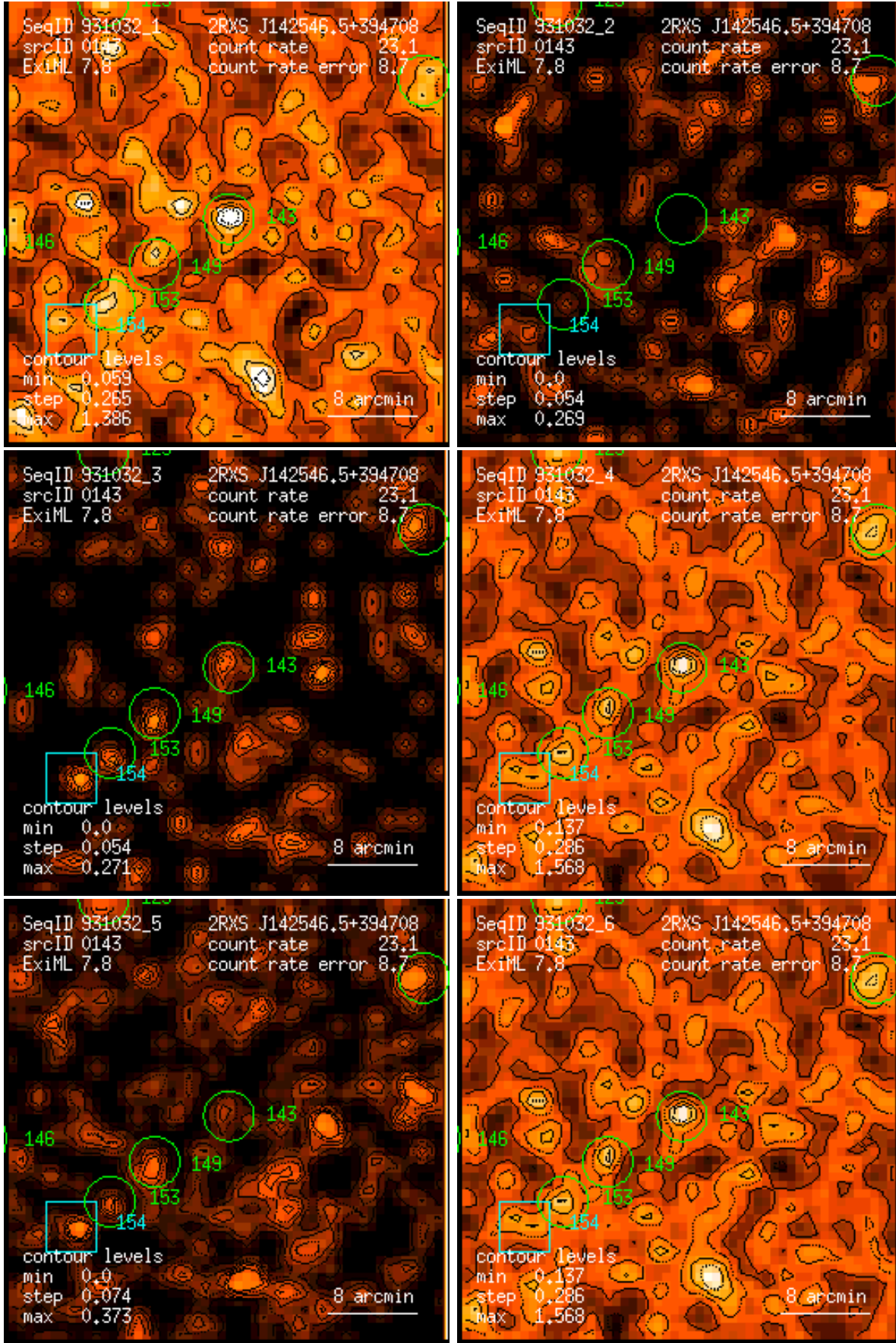
Figure 143: RASS 931032: detection 0143: band rate images, Gaussian filter: (1) PSPC channels 11 – 41, (2) 52 – 90, (3) 91 – 201, (4) 11 – 235, (5) 52 – 201, (6) 11 – 201. Broad band rates in counts/ks. Band rate contour levels in counts/ks/arcmin 2 .
