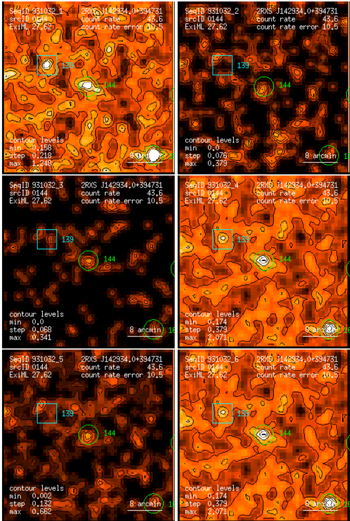
Figure 144: RASS 931032: detection 0144: band rate images, Gaussian filter: (1) PSPC channels 11 – 41, (2) 52 – 90, (3) 91 – 201, (4) 11 – 235, (5) 52 – 201, (6) 11 – 201. Broad band rates in counts/ks. Band rate contour levels in counts/ks/arcmin 2 .
