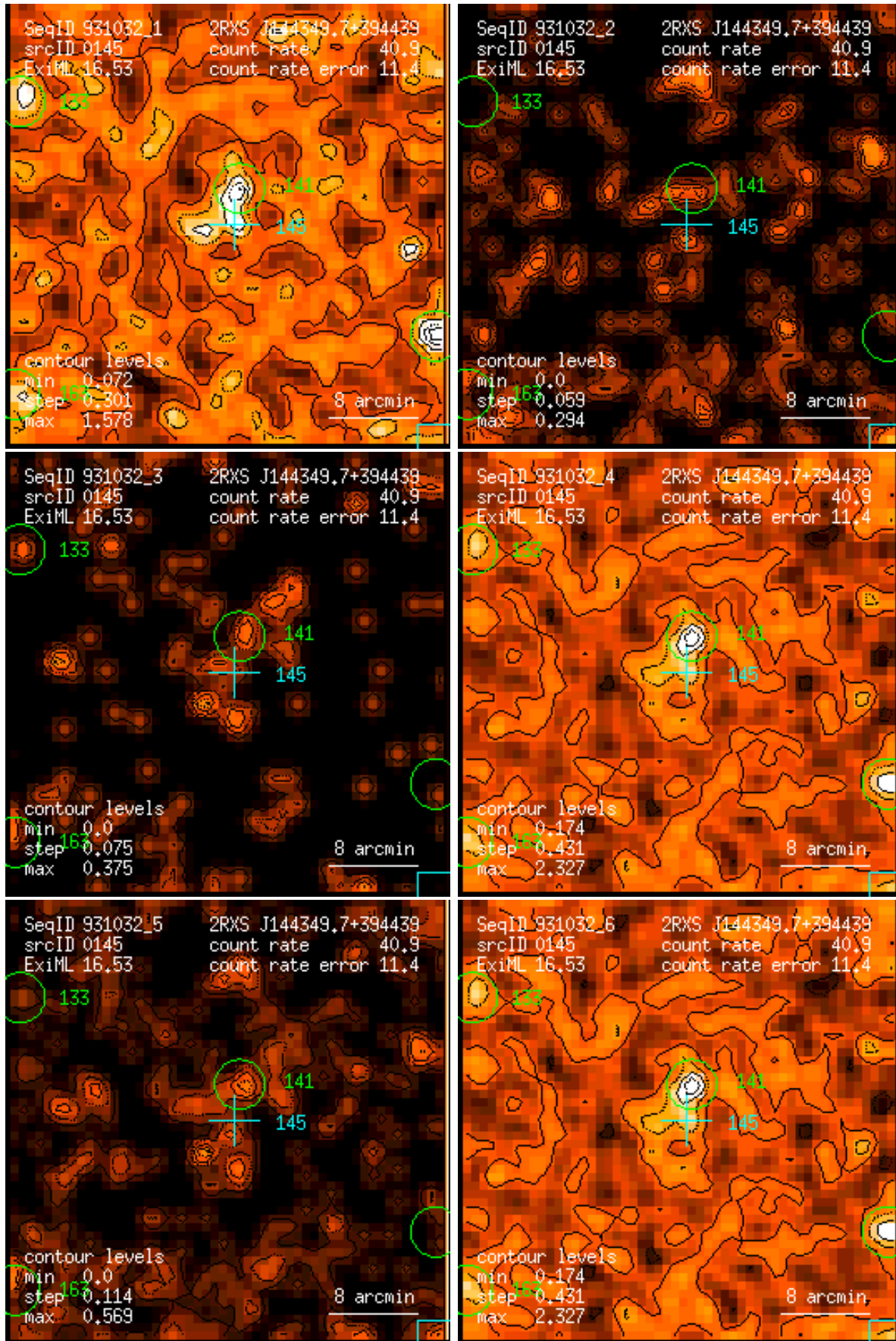
Figure 145: RASS 931032: detection 0145: band rate images, Gaussian filter: (1) PSPC channels 11 – 41, (2) 52 – 90, (3) 91 – 201, (4) 11 – 235, (5) 52 – 201, (6) 11 – 201. Broad band rates in counts/ks. Band rate contour levels in counts/ks/arcmin 2 .
