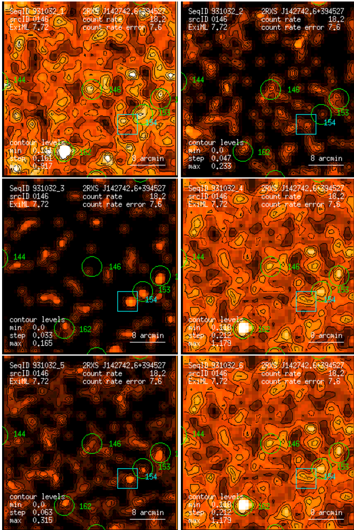
Figure 146: RASS 931032: detection 0146: band rate images, Gaussian filter: (1) PSPC channels 11 – 41, (2) 52 – 90, (3) 91 – 201, (4) 11 – 235, (5) 52 – 201, (6) 11 – 201. Broad band rates in counts/ks. Band rate contour levels in counts/ks/arcmin 2 .
