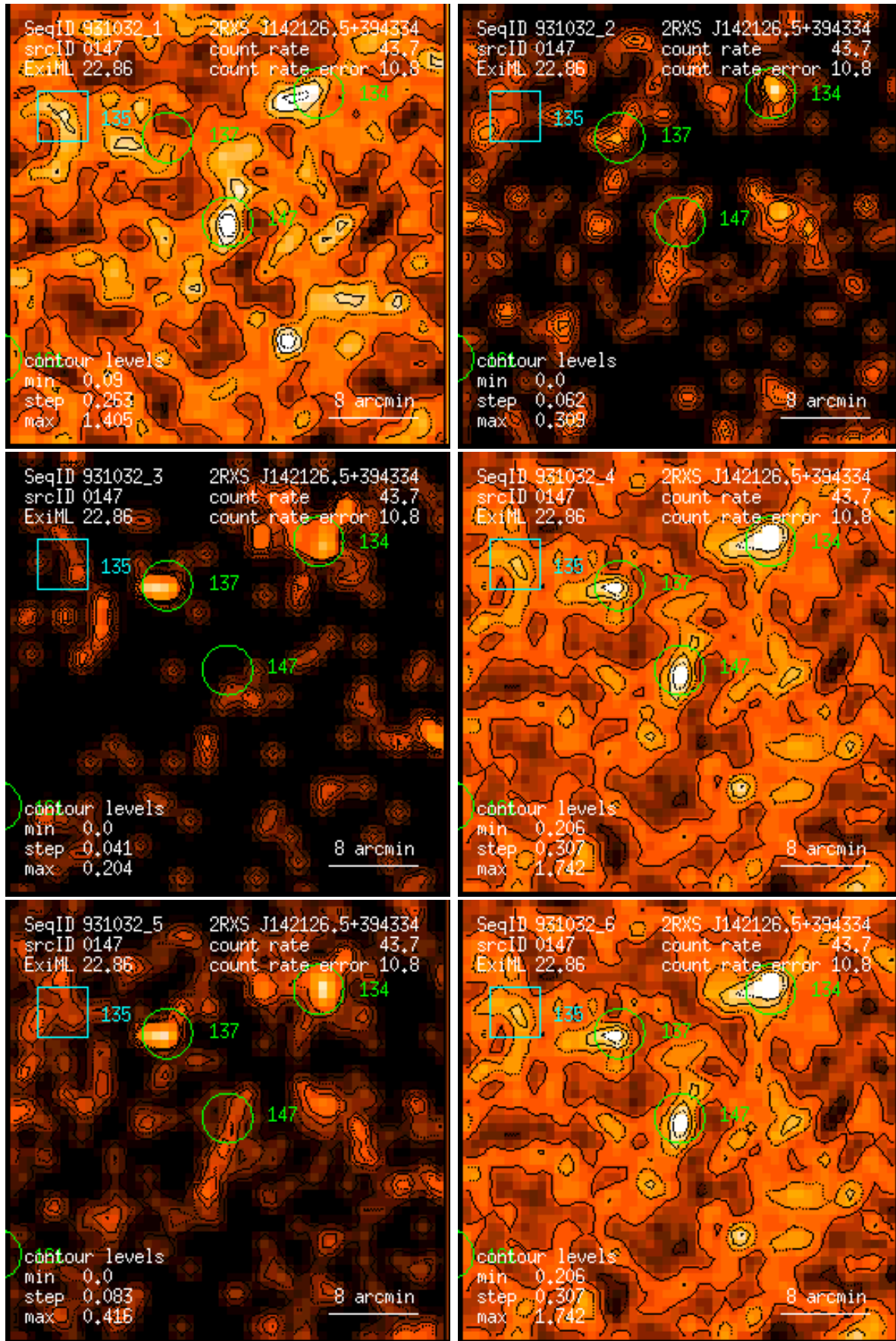
Figure 147: RASS 931032: detection 0147: band rate images, Gaussian filter: (1) PSPC channels 11 – 41, (2) 52 – 90, (3) 91 – 201, (4) 11 – 235, (5) 52 – 201, (6) 11 – 201. Broad band rates in counts/ks. Band rate contour levels in counts/ks/arcmin 2 .
