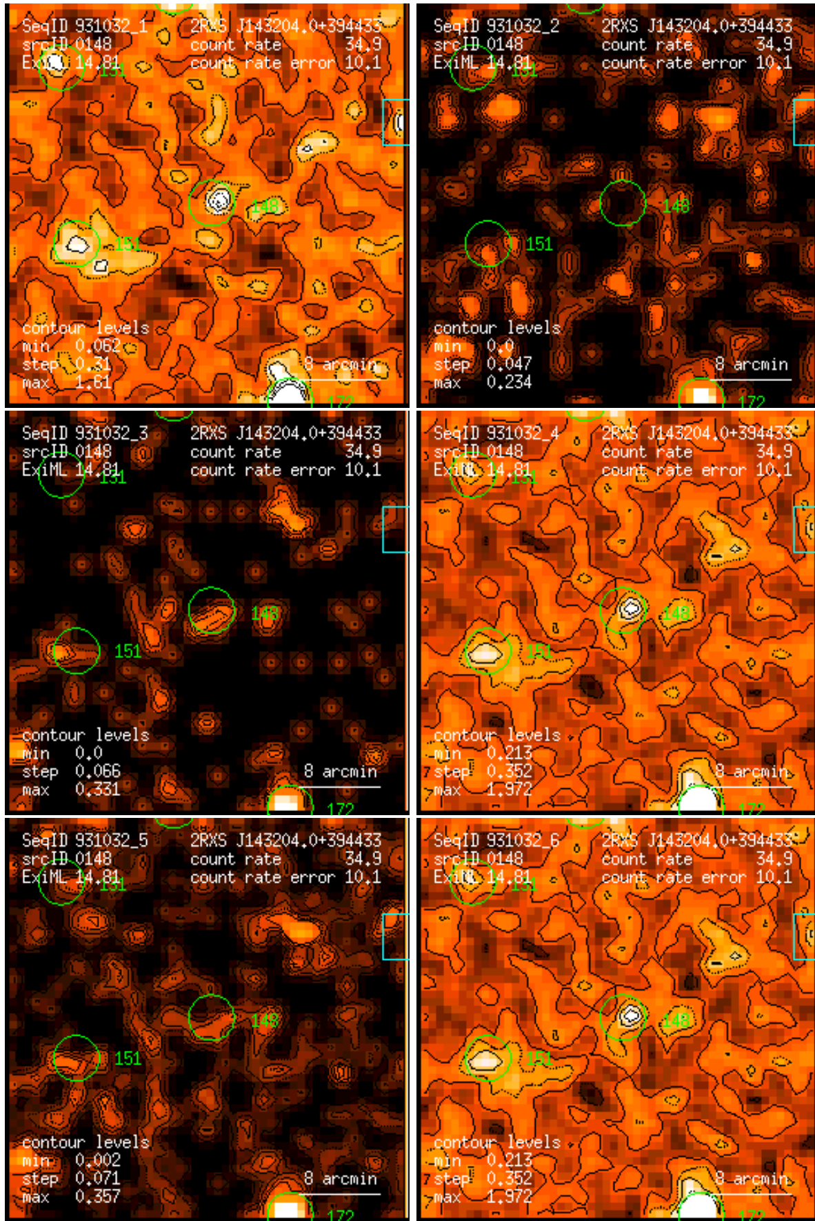
Figure 148: RASS 931032: detection 0148: band rate images, Gaussian filter: (1) PSPC channels 11 – 41, (2) 52 – 90, (3) 91 – 201, (4) 11 – 235, (5) 52 – 201, (6) 11 – 201. Broad band rates in counts/ks. Band rate contour levels in counts/ks/arcmin 2 .
