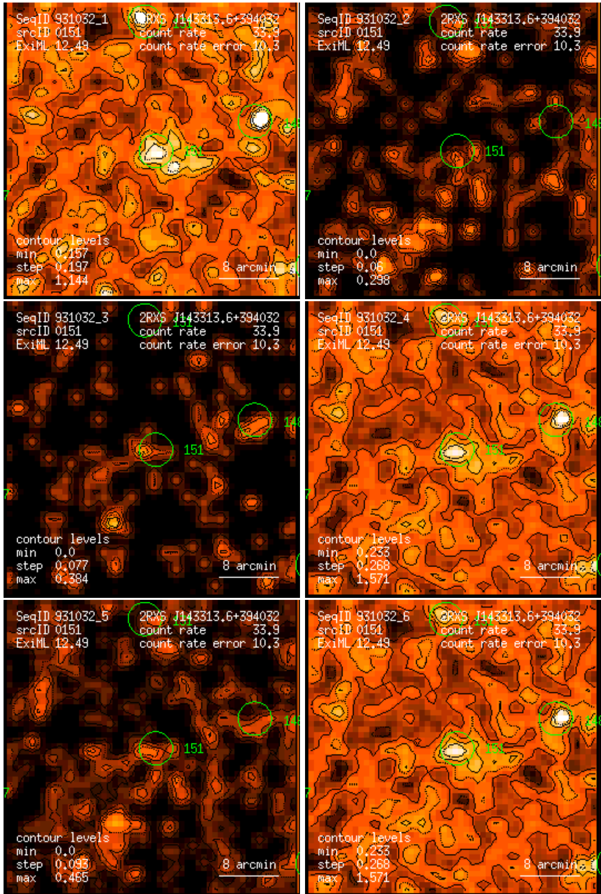
Figure 151: RASS 931032: detection 0151: band rate images, Gaussian filter: (1) PSPC channels 11 – 41, (2) 52 – 90, (3) 91 – 201, (4) 11 – 235, (5) 52 – 201, (6) 11 – 201. Broad band rates in counts/ks. Band rate contour levels in counts/ks/arcmin 2 .
