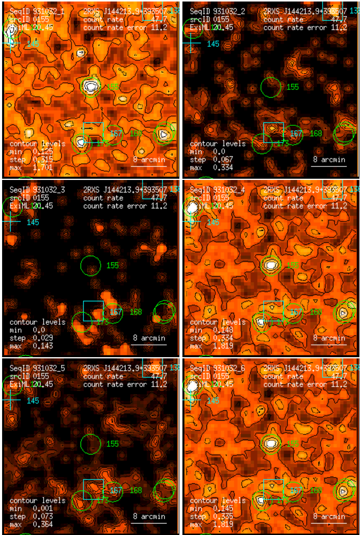
Figure 155: RASS 931032: detection 0155: band rate images, Gaussian filter: (1) PSPC channels 11 – 41, (2) 52 – 90, (3) 91 – 201, (4) 11 – 235, (5) 52 – 201, (6) 11 – 201. Broad band rates in counts/ks. Band rate contour levels in counts/ks/arcmin 2 .
