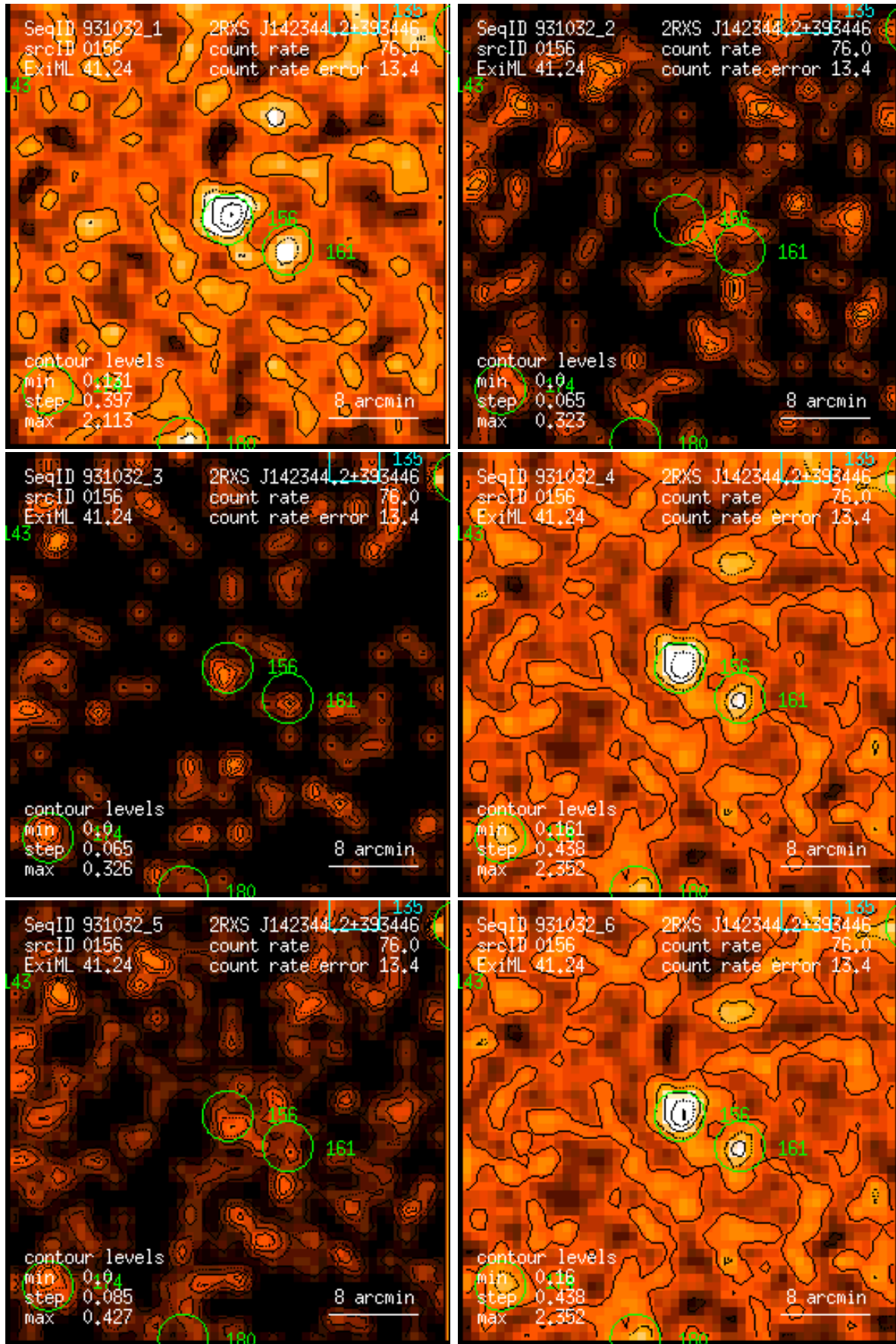
Figure 156: RASS 931032: detection 0156: band rate images, Gaussian filter: (1) PSPC channels 11 – 41, (2) 52 – 90, (3) 91 – 201, (4) 11 – 235, (5) 52 – 201, (6) 11 – 201. Broad band rates in counts/ks. Band rate contour levels in counts/ks/arcmin 2 .
