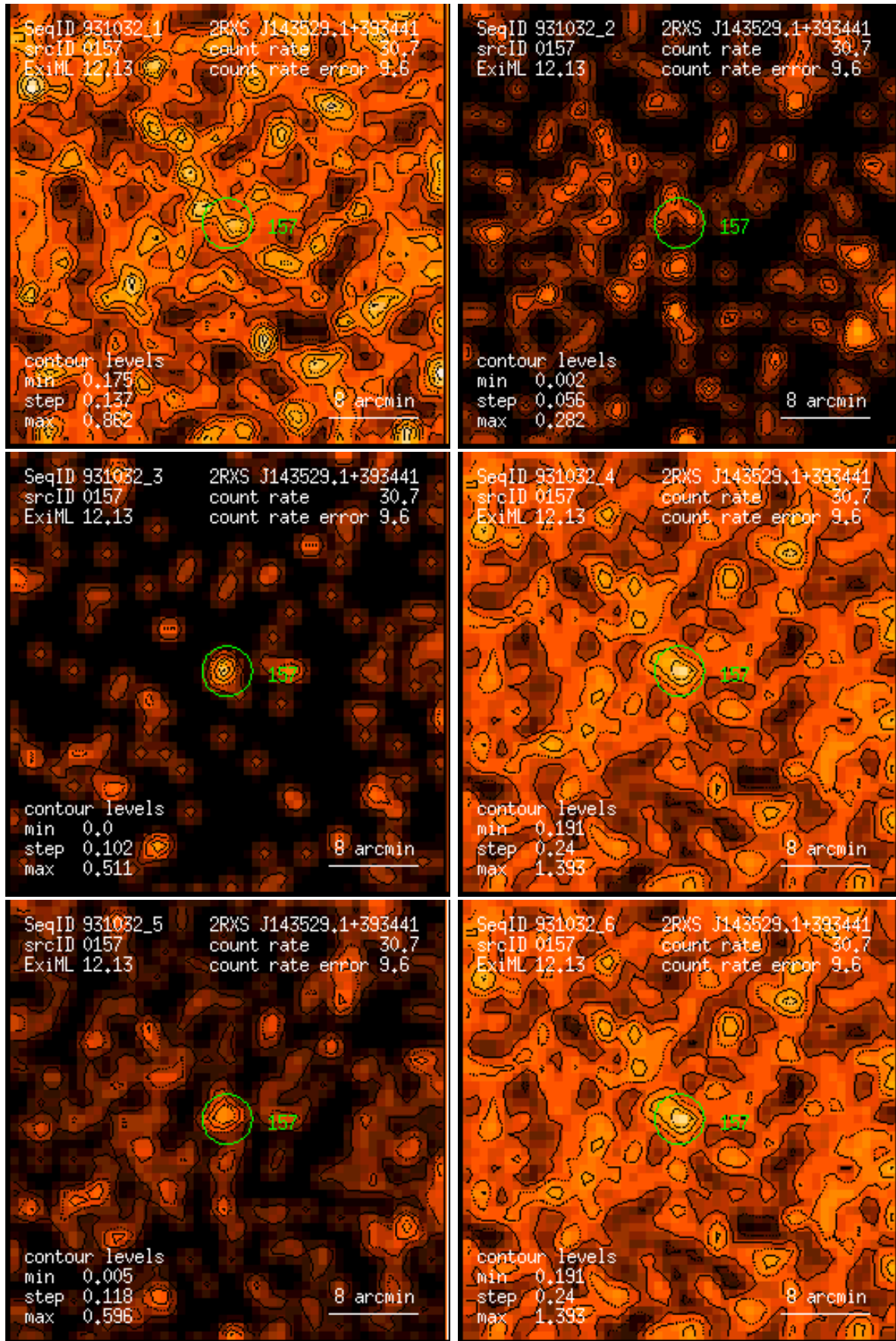
Figure 157: RASS 931032: detection 0157: band rate images, Gaussian filter: (1) PSPC channels 11 – 41, (2) 52 – 90, (3) 91 – 201, (4) 11 – 235, (5) 52 – 201, (6) 11 – 201. Broad band rates in counts/ks. Band rate contour levels in counts/ks/arcmin 2 .
