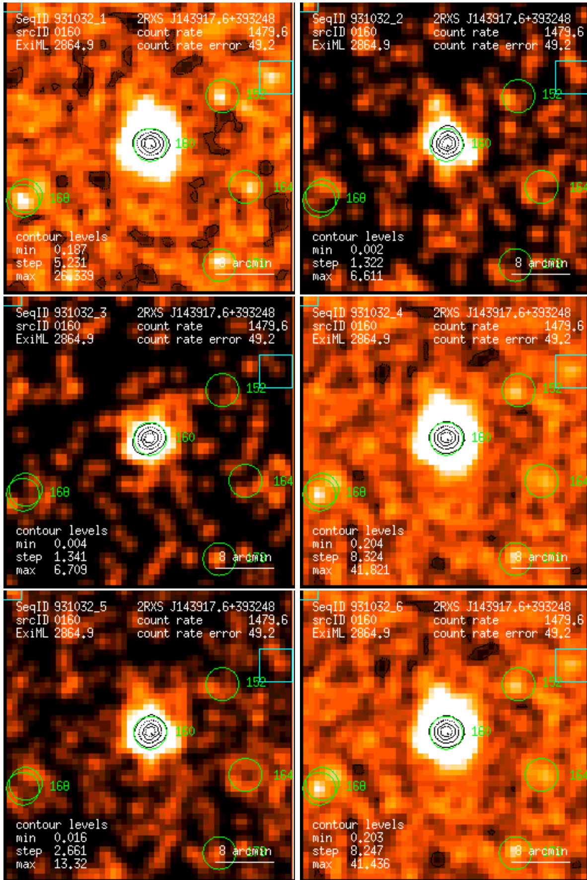
Figure 160: RASS 931032: detection 0160: band rate images, Gaussian filter: (1) PSPC channels 11 – 41, (2) 52 – 90, (3) 91 – 201, (4) 11 – 235, (5) 52 – 201, (6) 11 – 201. Broad band rates in counts/ks. Band rate contour levels in counts/ks/arcmin 2 .
