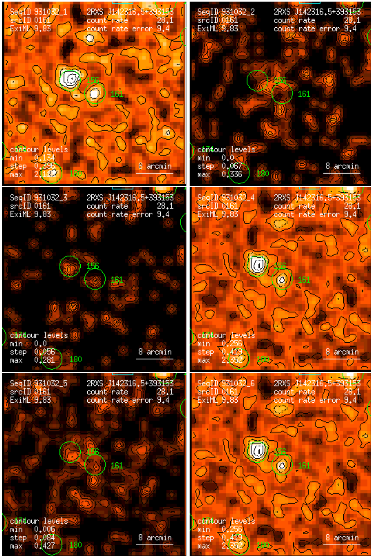
Figure 161: RASS 931032: detection 0161: band rate images, Gaussian filter: (1) PSPC channels 11 – 41, (2) 52 – 90, (3) 91 – 201, (4) 11 – 235, (5) 52 – 201, (6) 11 – 201. Broad band rates in counts/ks. Band rate contour levels in counts/ks/arcmin 2 .
