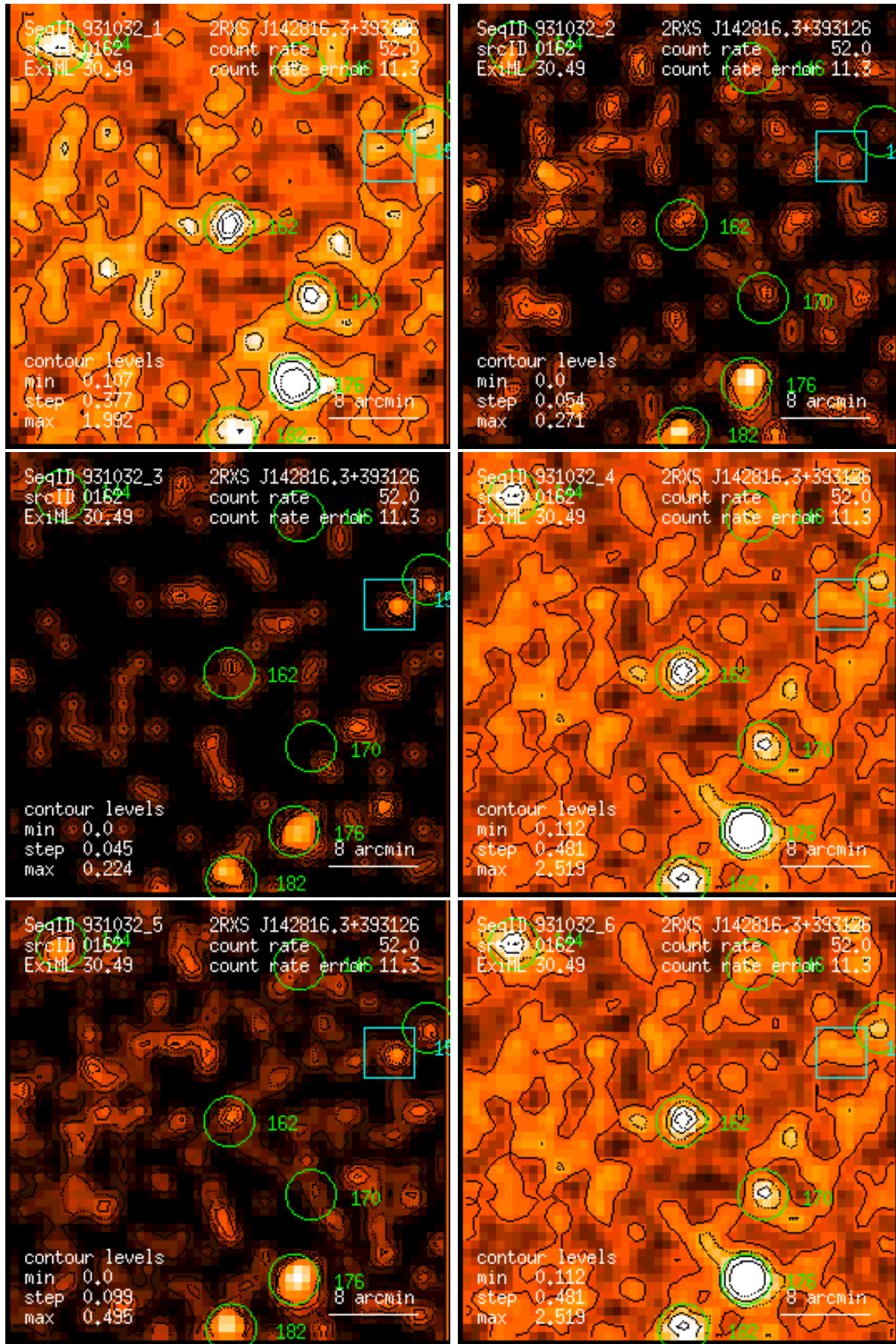
Figure 162: RASS 931032: detection 0162: band rate images, Gaussian filter: (1) PSPC channels 11 – 41, (2) 52 – 90, (3) 91 – 201, (4) 11 – 235, (5) 52 – 201, (6) 11 – 201. Broad band rates in counts/ks. Band rate contour levels in counts/ks/arcmin 2 .
