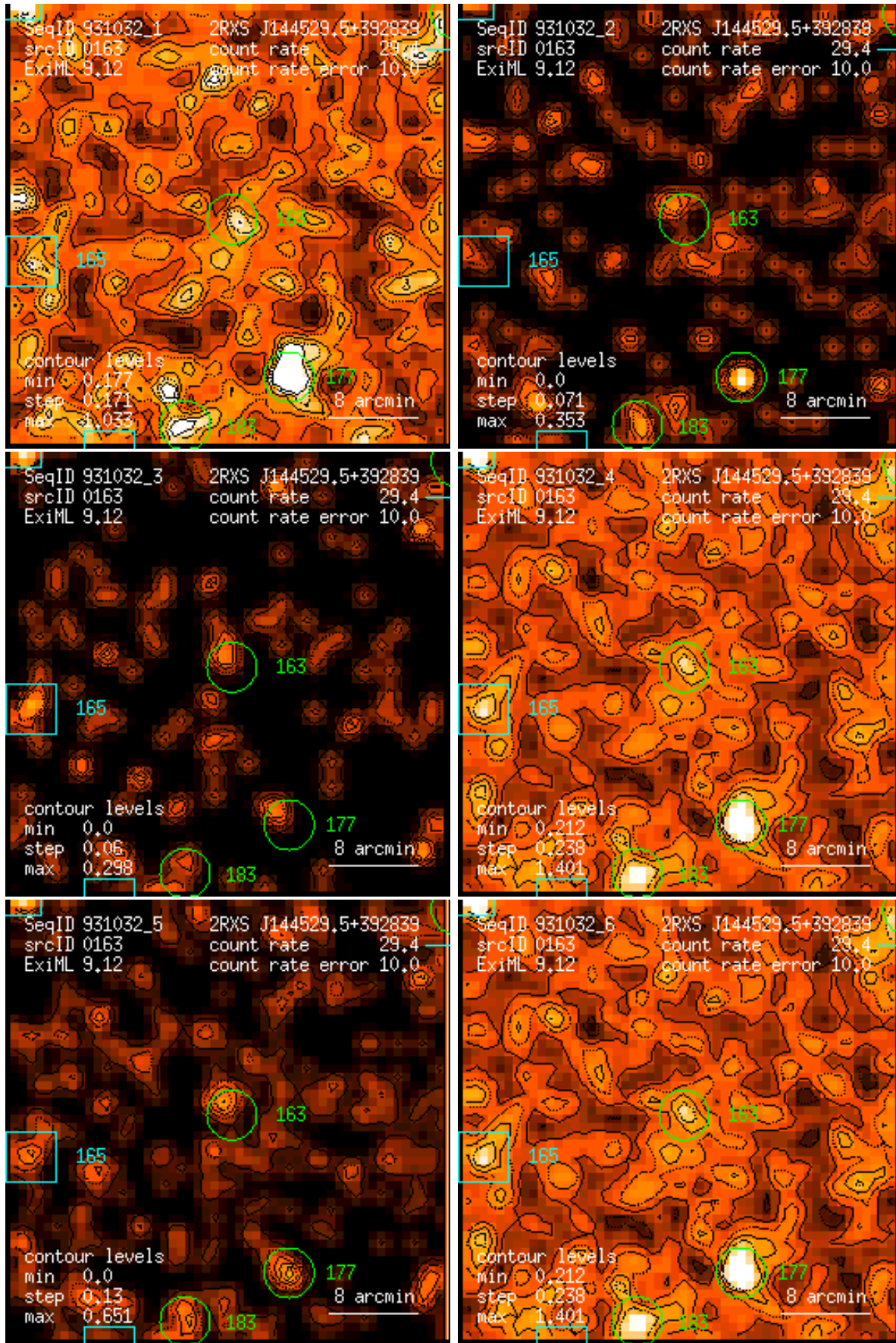
Figure 163: RASS 931032: detection 0163: band rate images, Gaussian filter: (1) PSPC channels 11 – 41, (2) 52 – 90, (3) 91 – 201, (4) 11 – 235, (5) 52 – 201, (6) 11 – 201. Broad band rates in counts/ks. Band rate contour levels in counts/ks/arcmin 2 .
