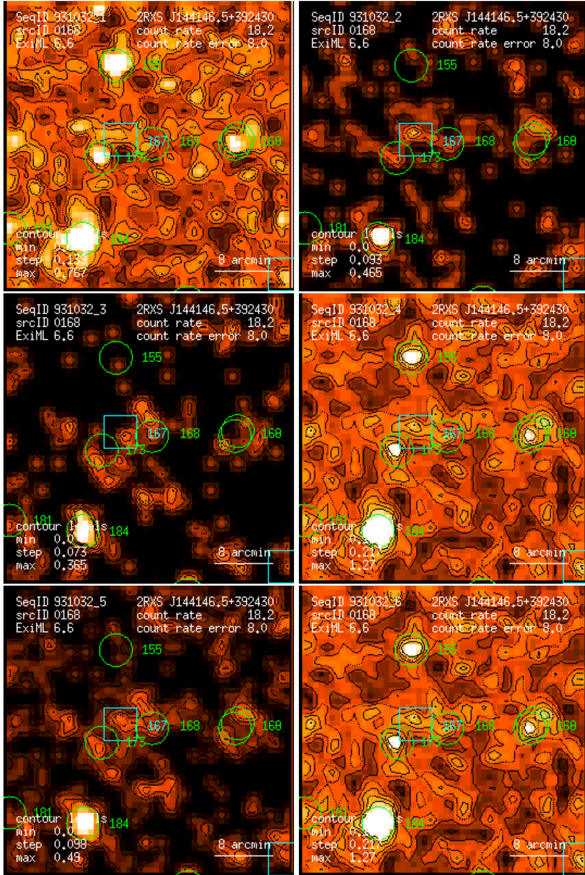
Figure 168: RASS 931032: detection 0168: band rate images, Gaussian filter: (1) PSPC channels 11 – 41, (2) 52 – 90, (3) 91 – 201, (4) 11 – 235, (5) 52 – 201, (6) 11 – 201. Broad band rates in counts/ks. Band rate contour levels in counts/ks/arcmin 2 .
