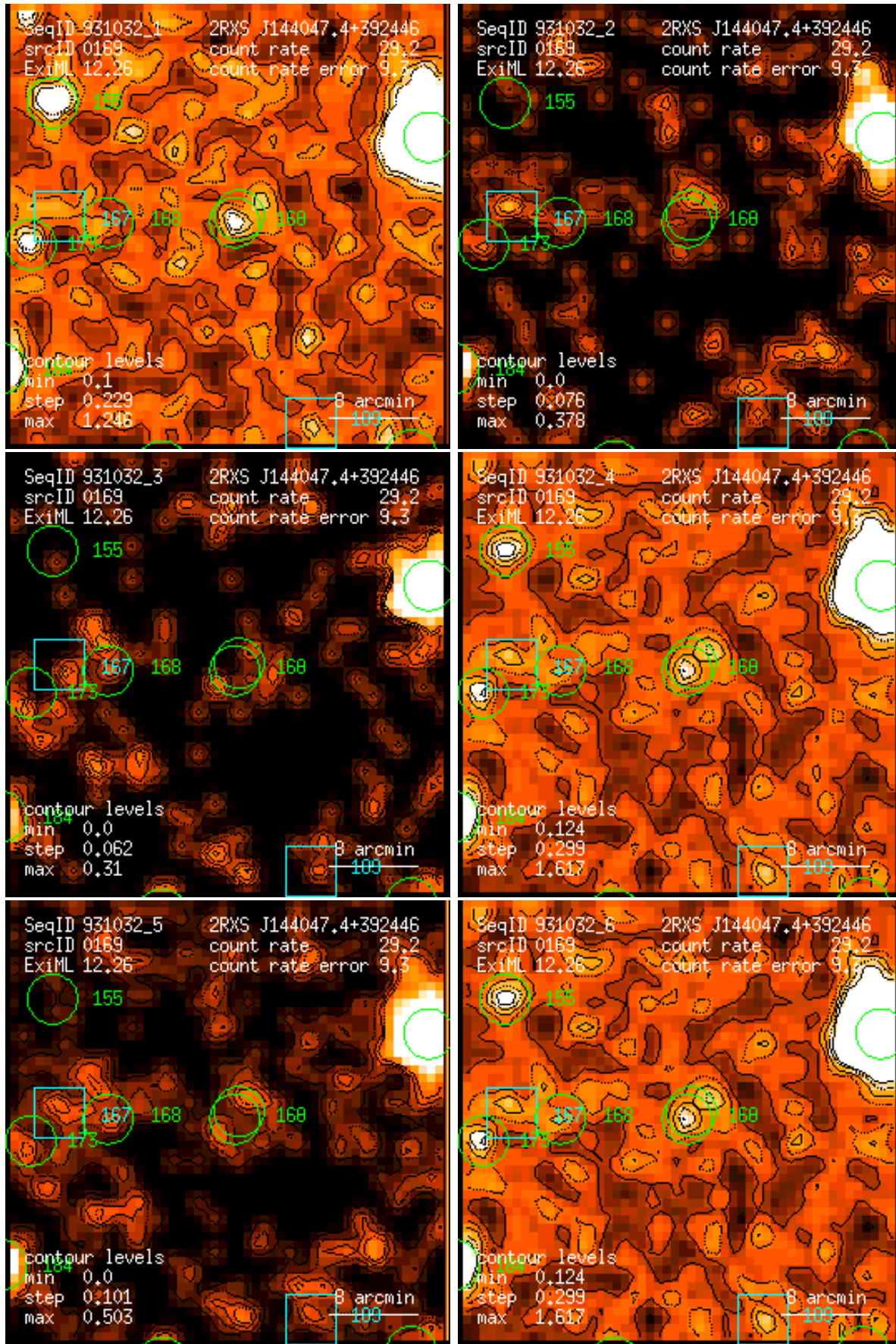
Figure 169: RASS 931032: detection 0169: band rate images, Gaussian filter: (1) PSPC channels 11 – 41, (2) 52 – 90, (3) 91 – 201, (4) 11 – 235, (5) 52 – 201, (6) 11 – 201. Broad band rates in counts/ks. Band rate contour levels in counts/ks/arcmin 2 .
