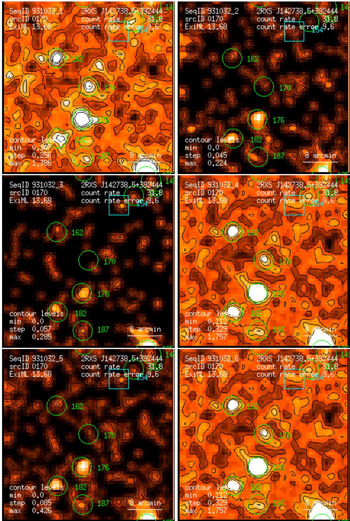
Figure 170: RASS 931032: detection 0170: band rate images, Gaussian filter: (1) PSPC channels 11 – 41, (2) 52 – 90, (3) 91 – 201, (4) 11 – 235, (5) 52 – 201, (6) 11 – 201. Broad band rates in counts/ks. Band rate contour levels in counts/ks/arcmin 2 .
