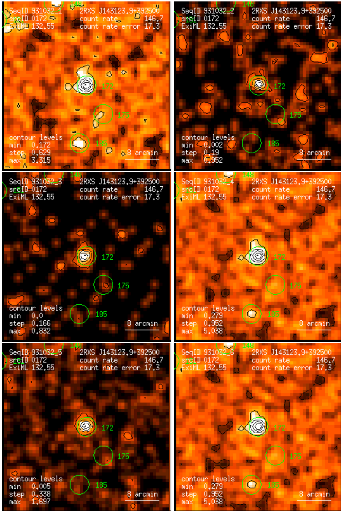
Figure 172: RASS 931032: detection 0172: band rate images, Gaussian filter: (1) PSPC channels 11 – 41, (2) 52 – 90, (3) 91 – 201, (4) 11 – 235, (5) 52 – 201, (6) 11 – 201. Broad band rates in counts/ks. Band rate contour levels in counts/ks/arcmin 2 .
