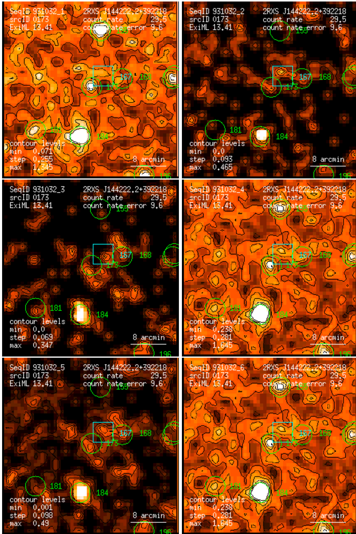
Figure 173: RASS 931032: detection 0173: band rate images, Gaussian filter: (1) PSPC channels 11 – 41, (2) 52 – 90, (3) 91 – 201, (4) 11 – 235, (5) 52 – 201, (6) 11 – 201. Broad band rates in counts/ks. Band rate contour levels in counts/ks/arcmin 2 .
