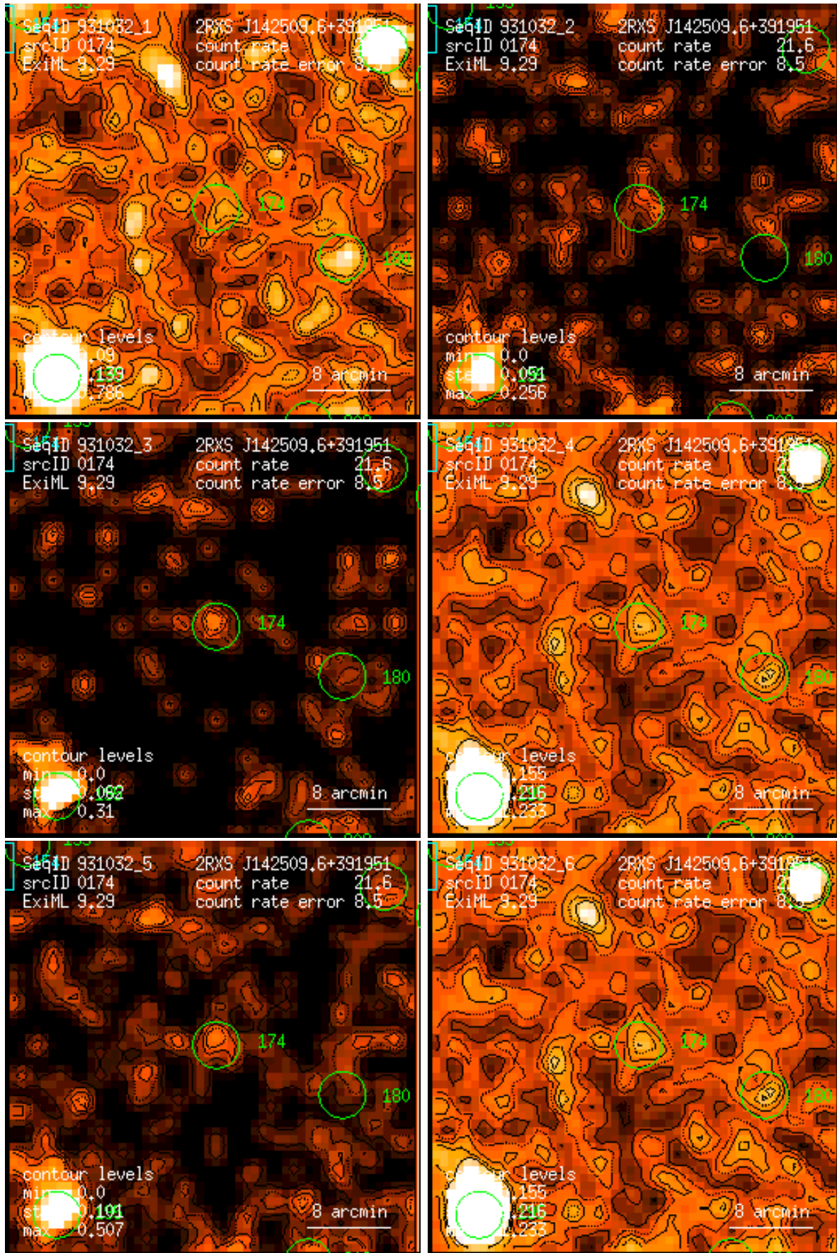
Figure 174: RASS 931032: detection 0174: band rate images, Gaussian filter: (1) PSPC channels 11 – 41, (2) 52 – 90, (3) 91 – 201, (4) 11 – 235, (5) 52 – 201, (6) 11 – 201. Broad band rates in counts/ks. Band rate contour levels in counts/ks/arcmin 2 .
