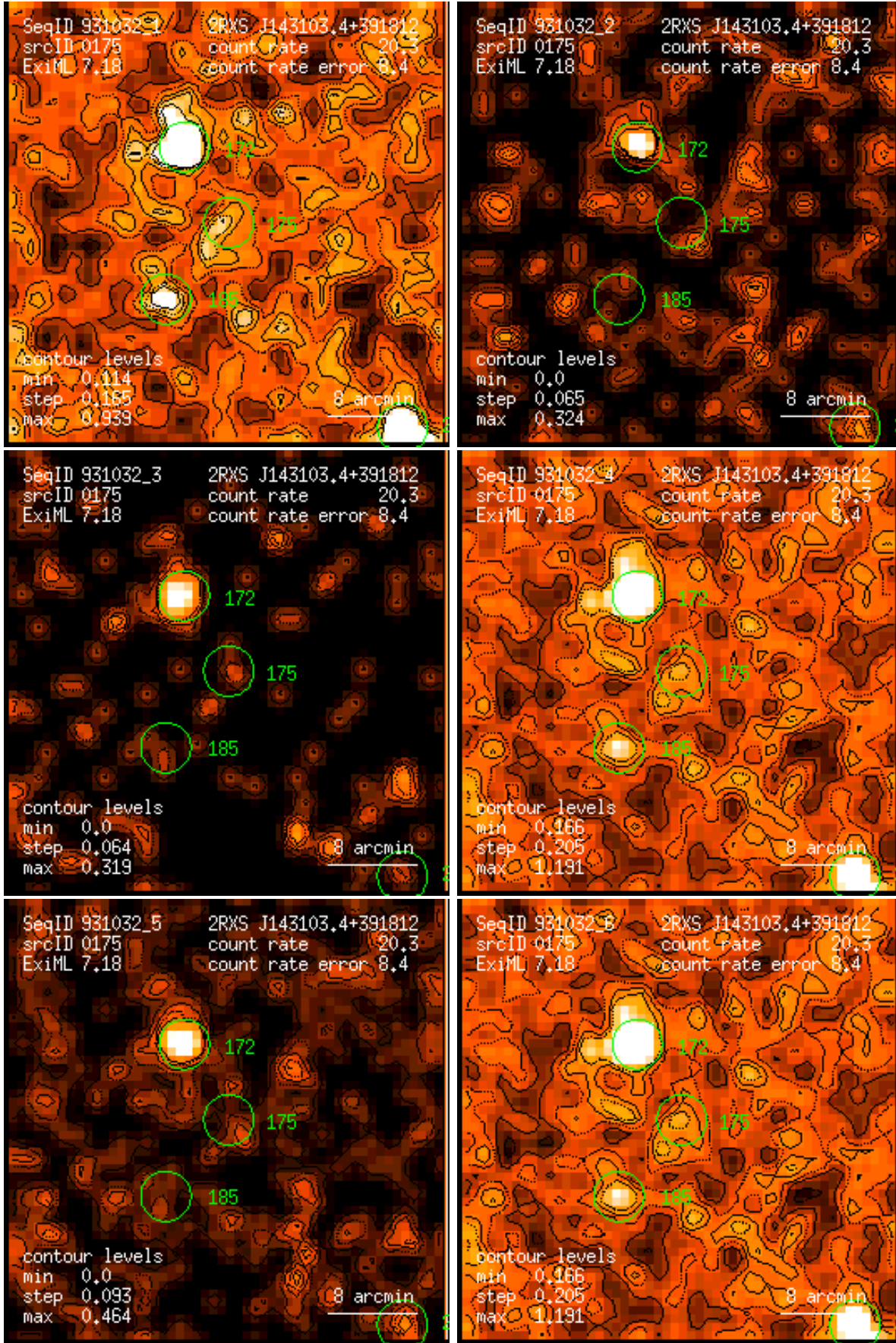
Figure 175: RASS 931032: detection 0175: band rate images, Gaussian filter: (1) PSPC channels 11 – 41, (2) 52 – 90, (3) 91 – 201, (4) 11 – 235, (5) 52 – 201, (6) 11 – 201. Broad band rates in counts/ks. Band rate contour levels in counts/ks/arcmin 2 .
