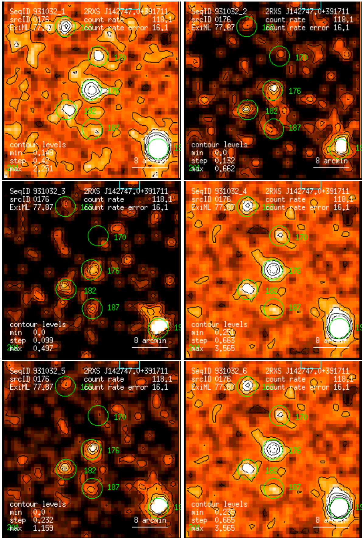
Figure 176: RASS 931032: detection 0176: band rate images, Gaussian filter: (1) PSPC channels 11 – 41, (2) 52 – 90, (3) 91 – 201, (4) 11 – 235, (5) 52 – 201, (6) 11 – 201. Broad band rates in counts/ks. Band rate contour levels in counts/ks/arcmin 2 .
