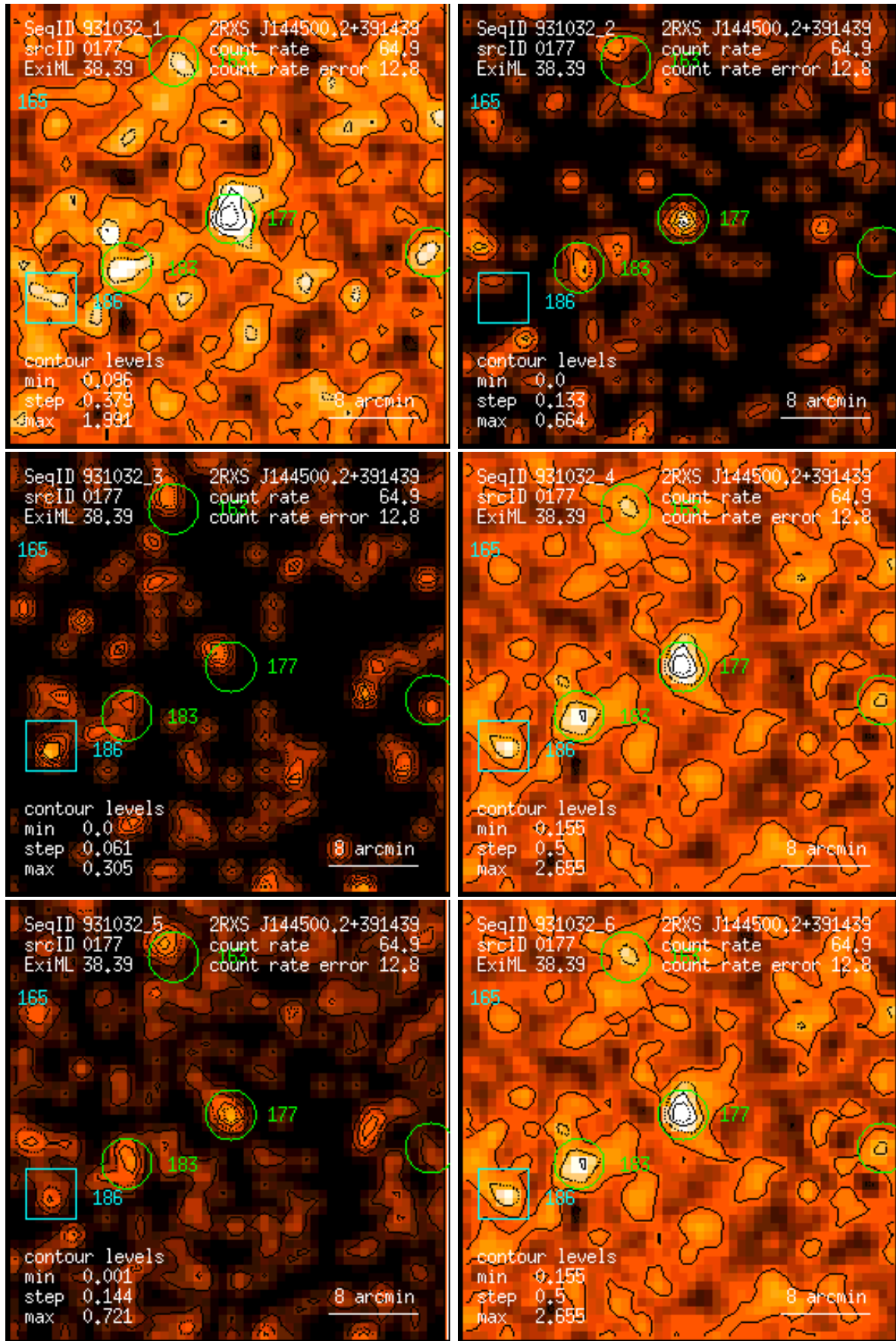
Figure 177: RASS 931032: detection 0177: band rate images, Gaussian filter: (1) PSPC channels 11 – 41, (2) 52 – 90, (3) 91 – 201, (4) 11 – 235, (5) 52 – 201, (6) 11 – 201. Broad band rates in counts/ks. Band rate contour levels in counts/ks/arcmin 2 .
