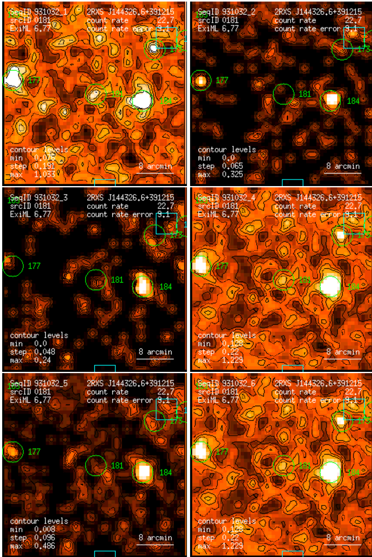
Figure 181: RASS 931032: detection 0181: band rate images, Gaussian filter: (1) PSPC channels 11 – 41, (2) 52 – 90, (3) 91 – 201, (4) 11 – 235, (5) 52 – 201, (6) 11 – 201. Broad band rates in counts/ks. Band rate contour levels in counts/ks/arcmin 2 .
