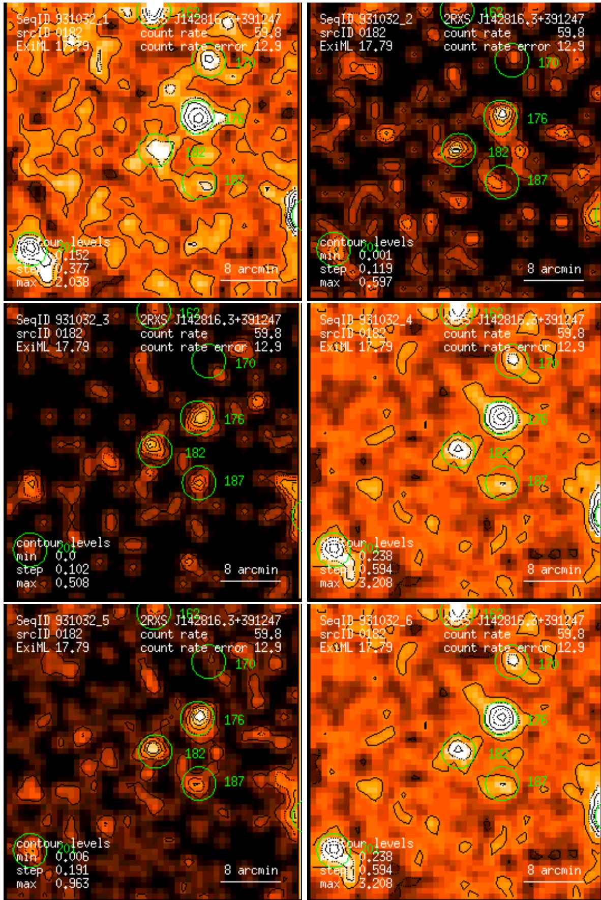
Figure 182: RASS 931032: detection 0182: band rate images, Gaussian filter: (1) PSPC channels 11 – 41, (2) 52 – 90, (3) 91 – 201, (4) 11 – 235, (5) 52 – 201, (6) 11 – 201. Broad band rates in counts/ks. Band rate contour levels in counts/ks/arcmin 2 .
